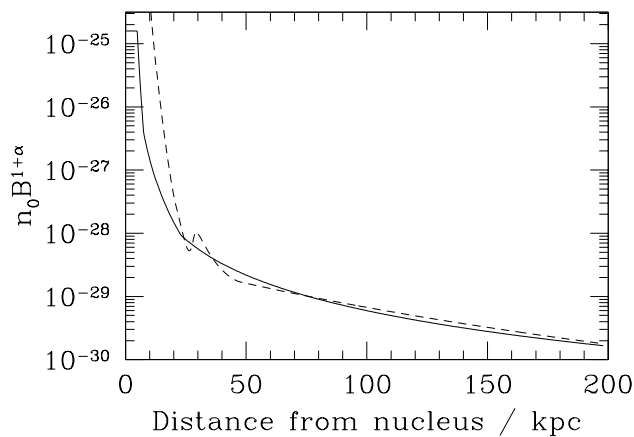
Figure 13: Profiles of n_0 B^{1+\alpha} for 1553+24, from Canvin & Laing (2004). The units are as in Fig. 6. The full line shows the results from the free model and the dashed line the adiabatic model prediction, normalised to match at large distances from the nucleus. Note the good agreement over a factor of 20 in distance and 50 in emissivity.
