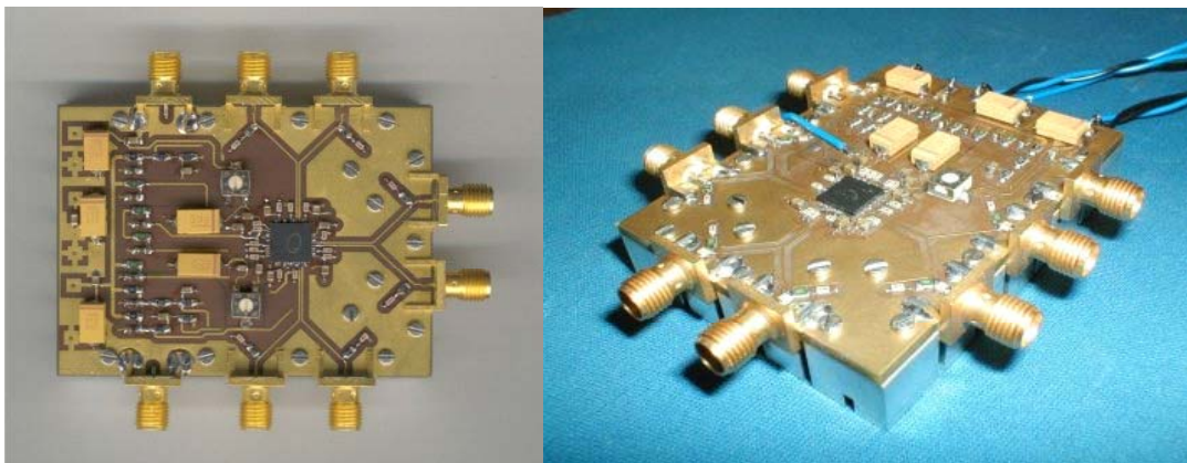
Figure 18. 3-bit Sampler
