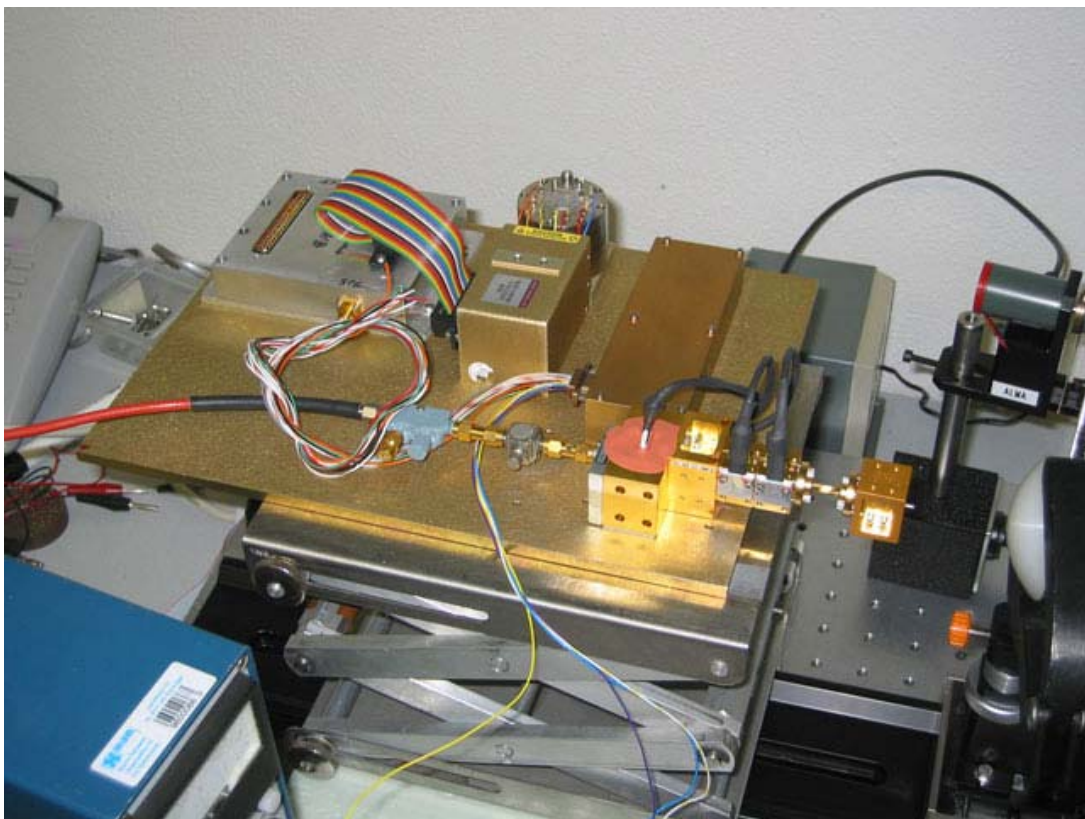
Figure 16. ALMA pre-prototype Band 9 local oscillator mounted at FTS test bench at SRON
