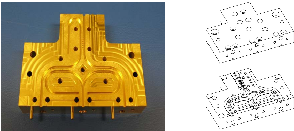
Figure 8. Band 3 quadrature hybrid
