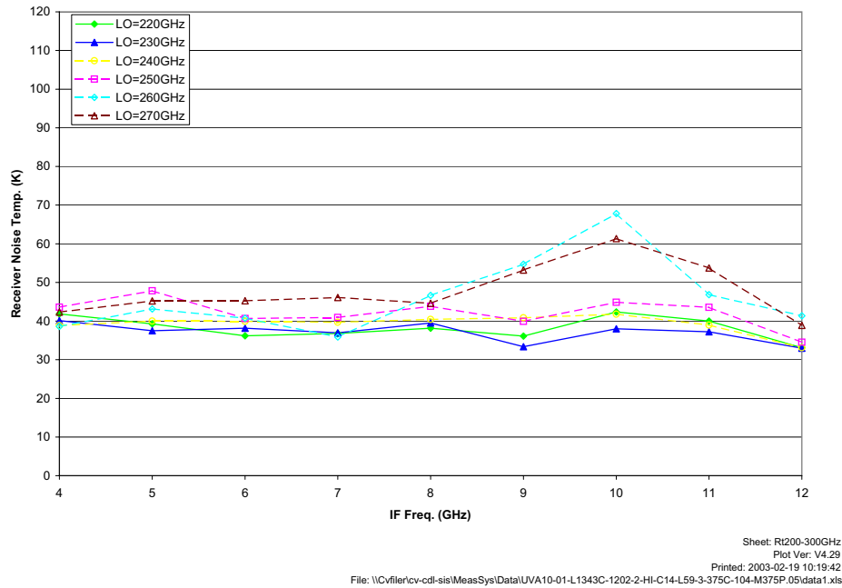
Figure 10. Band 6 receiver performance; ALMA spec 39K
