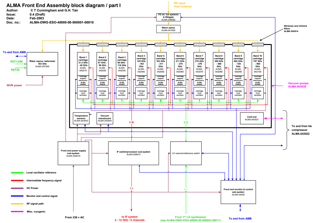
Figure 14. Receiver block diagram
