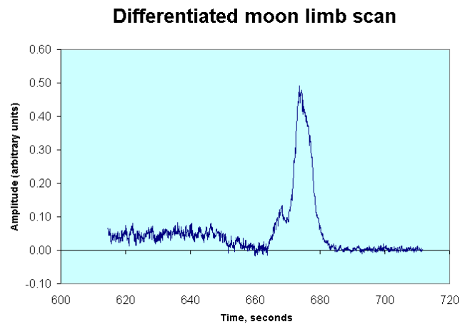
Figure 12b. Data from evaluation receiver #1 at 100 GHz
