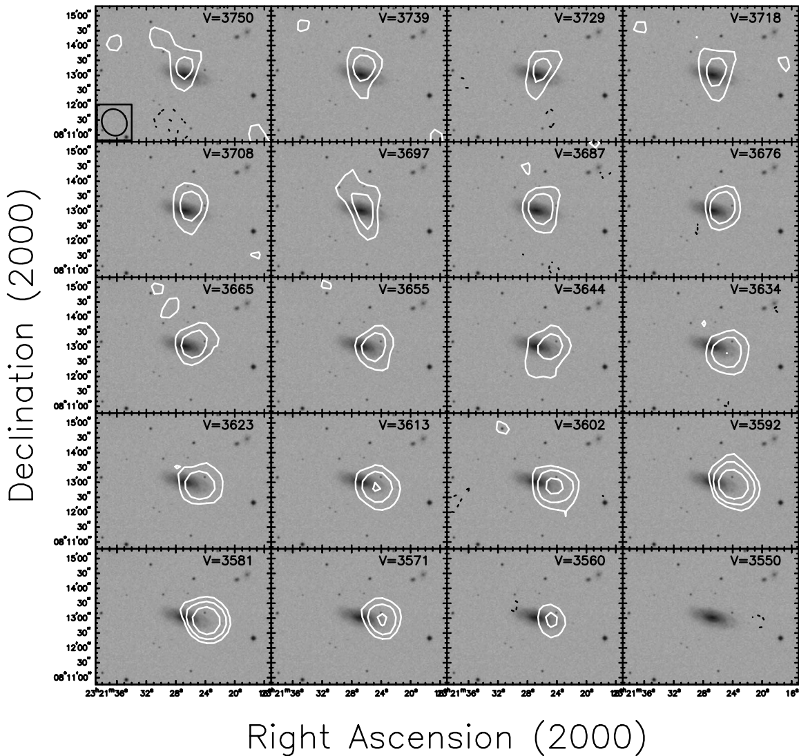
FIG. 11.—H I contours upon optical image from the DSS for H I channel maps contoured upon a gray-scale representation of the DSS optical image for NGC 7631, the companion lying 11' ( 145 kpc) to the east to NGC 7626. The heliocentric velocity of each channel is given at upper right in each panel, and the size of the synthesized beam ( 55'' \times 49'' FWHM) is indicated by the inscribed ellipse at lower left in the first panel. Contours are drawn at levels of -3 , 3 , 6 , and 12 times 0.64 mJy beam ^{-1} , where the lowest contour corresponds to an H I column density of 8.2 \times 10^{18} cm ^{-2} .
