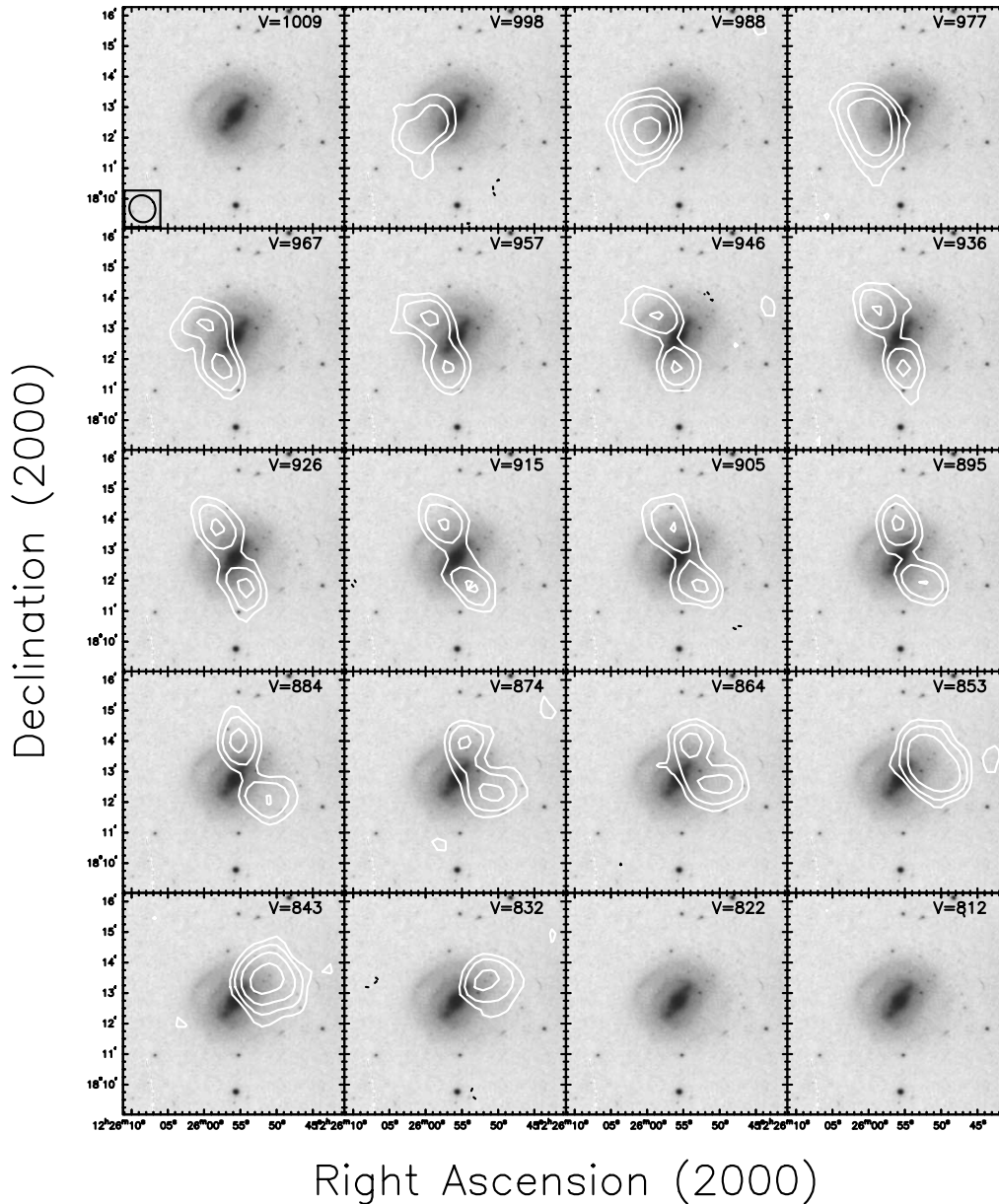
FIG. 4.—H I channel maps contoured upon a gray-scale representation of the DSS optical image for NGC 4394, the barred companion lying 7\frac{1}{6} (37 kpc) to the east of NGC 4382. The heliocentric velocity of each channel is given at upper right in each panel, and the size of the synthesized beam ( 54'' \times 50'' FWHM) is indicated by the inscribed ellipse at lower left in the first panel. Contours are drawn at levels of -3, 3, 6, 12, and 24 times 0.76 mJy beam ^{-1} , where the lowest contour corresponds to an H I column density of 9.8 \times 10^{18} cm ^{-2} .
