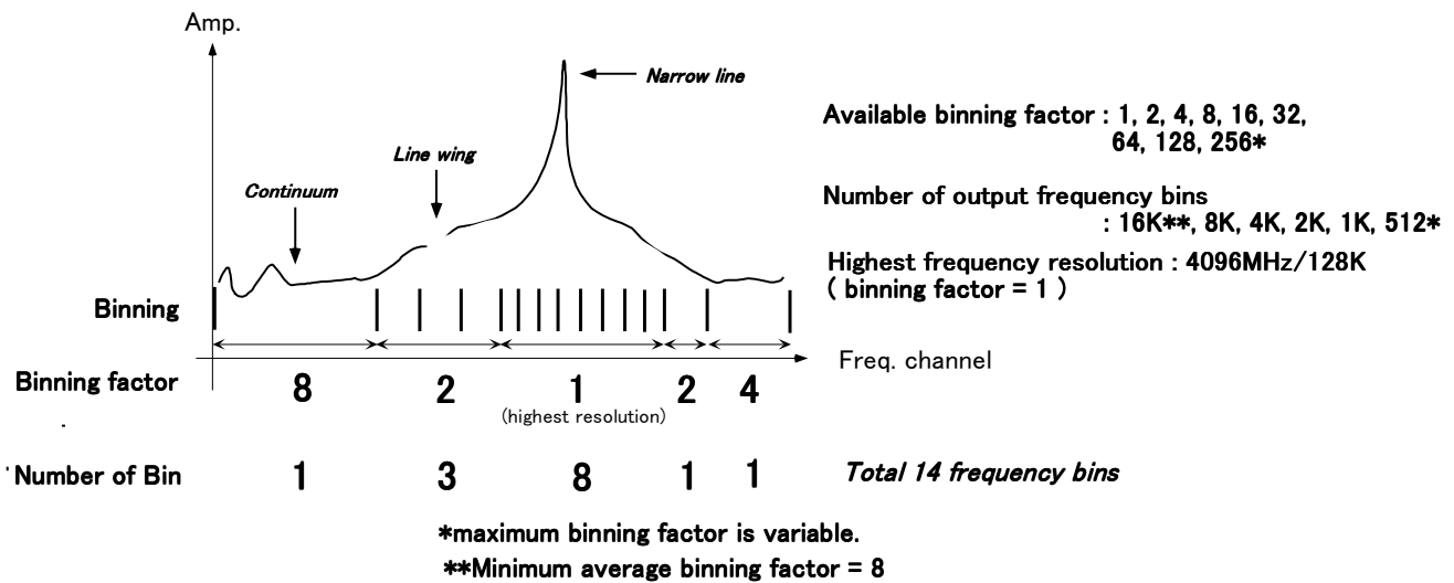
Figure 5. Example of the flexible frequency-region smoothing.
