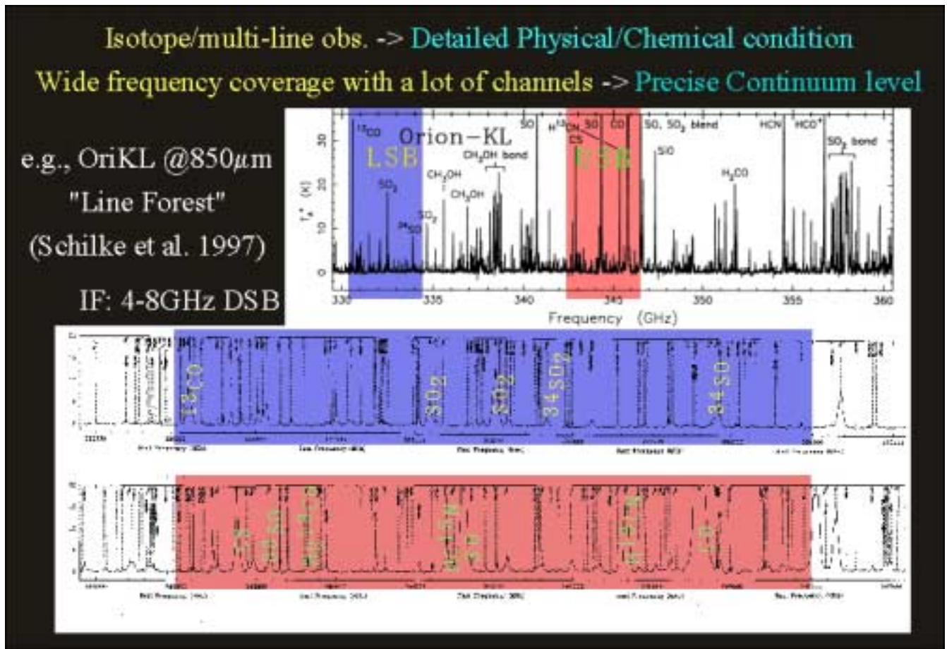
Figure 1. Orion KL wideband spectra at 850micron 2 .
