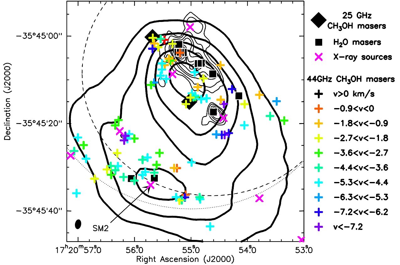
Fig. 4.— SMA 1.3 mm continuum contours of I(N) (thin black contours) with thick black contours showing SCUBA 450 \mu\text{m} emission (G. Sandell, private communication). The 1.3 mm continuum image and contour levels are the same as Fig. 1. The SCUBA 450 \mu\text{m} resolution is 8'' and the contour levels are 60, 80, 100, 120, 160 \text{Jy beam}^{-1} . The tip of the arrow for SM2 is the position reported by Sandell (2000). The colored crosses show the locations of 44 GHz Class I methanol masers from this work. The locations of the water maser groups (also see Fig. 1) are shown by \blacksquare symbols and the 25 GHz \text{CH}_3\text{OH} masers reported by Beuther et al. (2005) are shown by \blacklozenge symbols. The X-ray sources from Feigelson et al. (2009) are marked by magenta X's. The dashed arc indicates the SMA primary beam and the dotted arc indicates the VLA 44 GHz primary beam. The 1.3 mm SMA continuum resolution is shown in the lower left.
