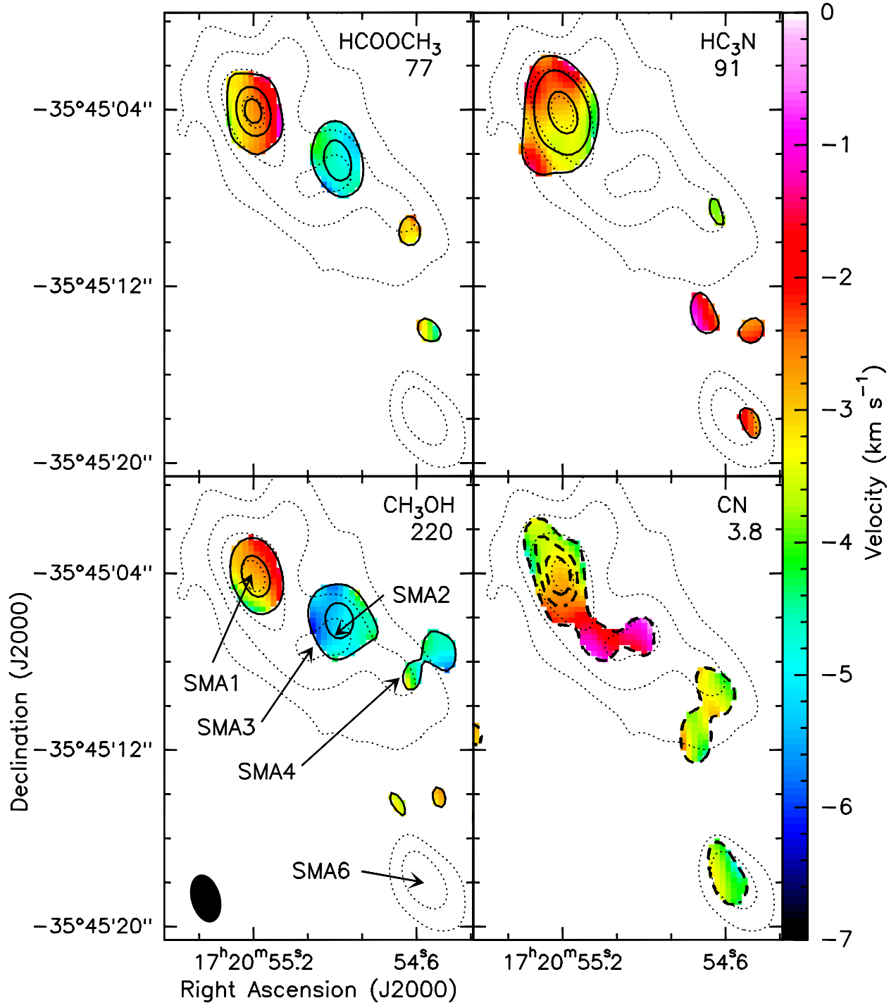
Fig. 9.— In each panel, the color scale shows the first moment map of the indicated molecular line, while the solid black contours depict the integrated intensity image of the line emission. In the case of \text{CN} , the dashed contours indicate that the line appears in absorption. The levels are: \text{HCOOCH}_3 = 2.1, 6.3, 10.5 \text{ Jy km s}^{-1} ; \text{HC}_3\text{N} = 2.55, 5.95, 14.45 \text{ Jy km s}^{-1} ; \text{CH}_3\text{OH} = 1.89, 5.67 \text{ Jy km s}^{-1} ; \text{CN} = -1.2, -2.4, -3.6 \text{ Jy km s}^{-1} . In each panel, the thin dotted contours show the 1.3 mm continuum emission (levels = 60, 180, 390, and 900 \text{mJy beam}^{-1} ). The numbers below each molecular name is the E_{\text{lower}} of the transition in units of \text{cm}^{-1} .
