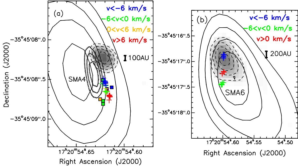
Fig. 3.— (a) Zoom of the SMA4 region with the grayscale and dashed contours showing the 1.3 cm continuum emission, dotted contours showing 3.6 cm, and the solid contours showing the uniformly weighted 1.3 mm continuum. The 3.6 cm contours are 0.12, 0.16, and 0.20 mJy beam -1 , the 1.3 cm contour levels are 0.19, 0.25, 0.31, and 0.37 mJy beam -1 , and the 1.3 mm contour levels are 100, 120, 140, and 160 mJy beam -1 . (b) Zoom of the SMA6 region with the grayscale and dashed contours showing 7 mm continuum emission and the solid contours showing the 1.3 mm continuum. The 7 mm contour levels are 0.6, 0.8, 1.0, and 1.2 mJy beam -1 , and the uniformly weighted 1.3 mm contour levels are 100, 140, 180, 220, and 260 mJy beam -1 . The cross symbols show the C5 (a) and C3 (b) water maser positions with S/N ratio > 7, color-coded by velocity. The filled square symbols in (a) show the location of 6.7 GHz CH 3 OH masers from Walsh et al. (1998), with same velocity coding as H 2 O masers.
