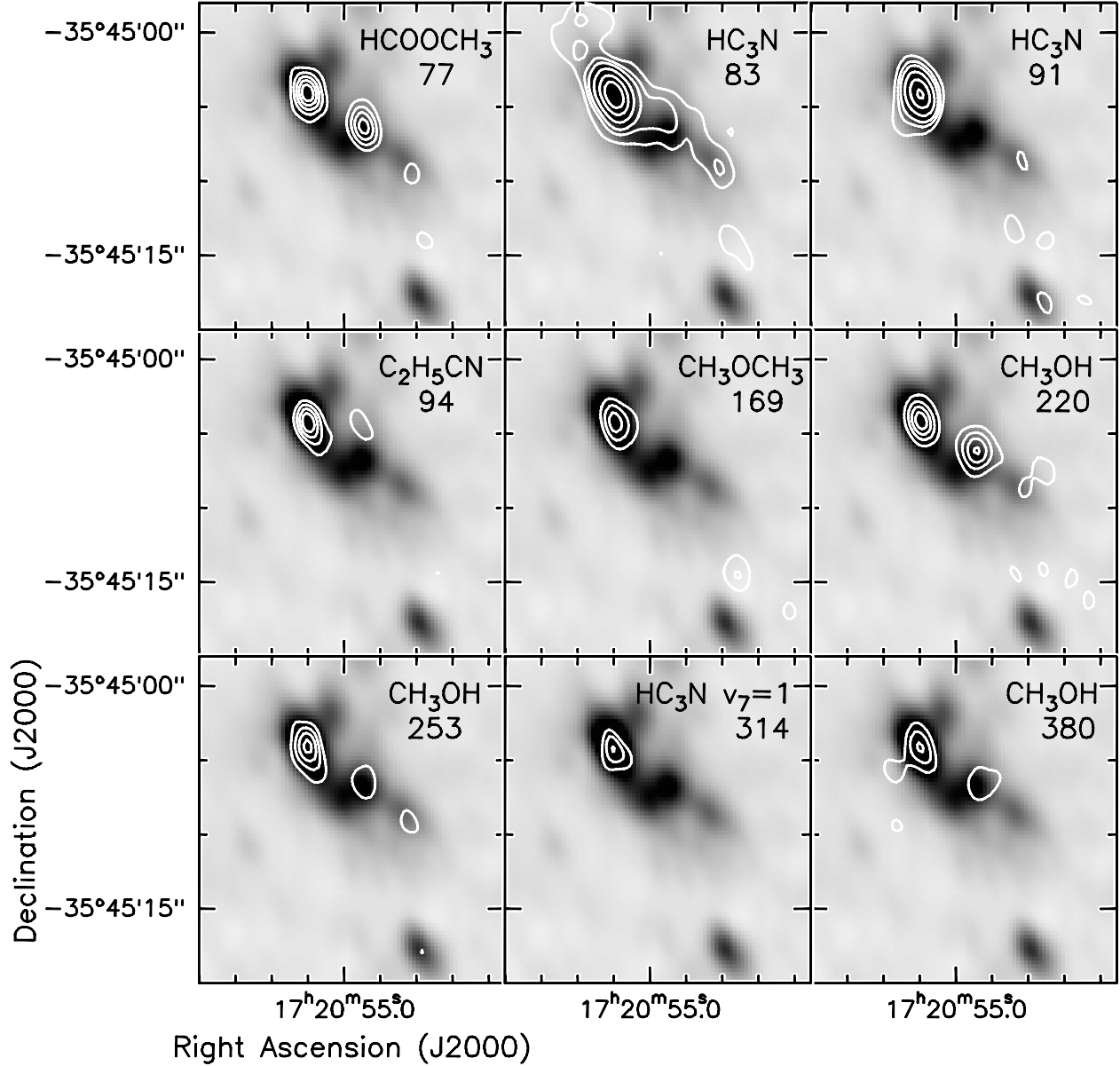
Fig. 8.— In each panel, the greyscale is the 1.3 mm continuum and the contours are drawn from moment-zero images of spectral lines. The contour levels are: HCOOCH 3 : 2.1, 4.2, 6.3, 8.4, 10.5 Jy km s -1 ; HC 3 N: 2.55, 4.25, 5.95, 9.35, 14.45, 19.55 Jy km s -1 ; C 2 H 5 CN: 1.8, 3.0, 4.2, 5.4 Jy km s -1 ; CH 3 OCH 3 : 1.35, 2.25, 3.15 Jy km s -1 ; CH 3 OH(220): 1.89, 3.78, 5.67, 7.56 Jy km s -1 ; 2.31, 3.85, 5.39, 6.93 Jy km s -1 ; HC 3 N(v 7 =1): 1.5, 2.5, 3.5 Jy km s -1 ; CH 3 OH(380): 2.1, 3.5, 4.9 Jy km s -1 . The numbers below each molecular name is the E_{\text{lower}} of the transition in units of cm -1 .
