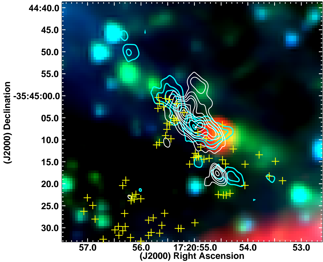
Fig. 11.— Spitzer 3-color image with RGB mapped to 24, 4.5, and 3.6 \mu\text{m} . White 1.3 mm continuum and cyan SiO integrated intensity contours are overlaid, along with yellow + symbols showing the locations of the 44 GHz \text{CH}_3\text{OH} masers. The 1.3 mm continuum contour levels are the same as Fig. 1, and the SiO (5–4) integrated emission contour levels are 6, 10, 14, 20, 26 \text{mJy beam}^{-1} \cdot \text{km s}^{-1} .
