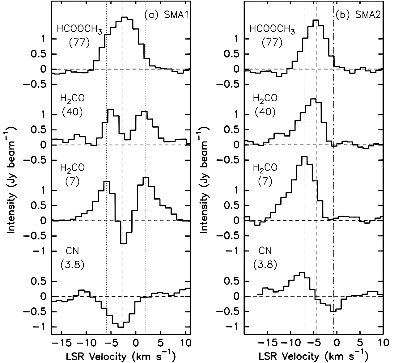
Fig. 10.— (a) Sample spectra toward the 1.3 mm continuum peak of SMA1. (b) Sample spectra toward the 1.3 mm continuum peak of SMA2. In both plots the dashed line indicates the V_{LSR} and the numbers in parenthesis under the molecule names are the lower state energy in \text{cm}^{-1} . In (a) the two dotted lines indicate the velocity of the peak red and blueshifted \text{H}_2\text{CO} ( E_l = 7 \text{ cm}^{-1} ) emission. In (b) the dotted line indicates the velocity of the peak blueshifted \text{H}_2\text{CO} ( E_l = 7 \text{ cm}^{-1} ) emission and the dot-dashed line indicates the velocity of maximum CN absorption.
