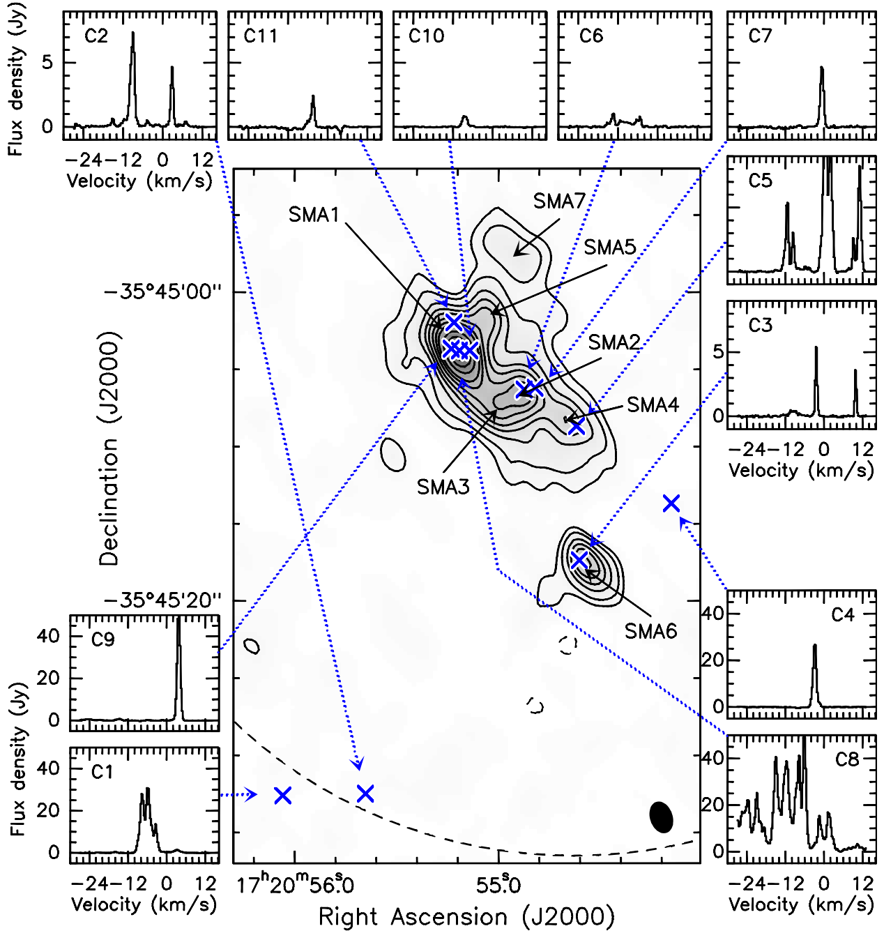
Fig. 1.— Composite image showing the naturally weighted SMA 1.3 mm continuum emission from I(N) with surrounding insets showing the VLA H 2 O (22.235 GHz) maser spectra. The 1.3 mm continuum image has a resolution of 2''.2 \times 1''.3 (P.A.=+15°) and the contour levels are 30 (3.5 \sigma ), 60, 120, 180, 240, 320, 400, 640, 800, 960 mJy beam -1 . The blue crosses show the intensity weighted centroid positions of the water maser groups listed in Table 2 (derived from Table 3). The water maser spectra show the average emission from each group. The dashed arc indicates the SMA primary beam, and the dashed arc indicates the VLA primary beam at 22 GHz. The 1.3 mm image has not been corrected for primary beam attenuation.
