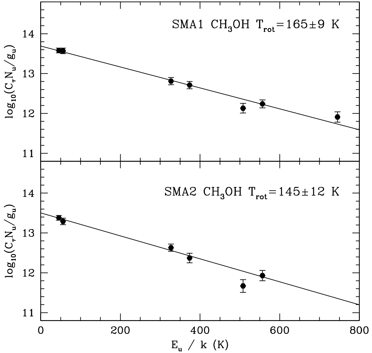
Fig. 12.— Rotation diagrams for the CH 3 OH transitions observed for SMA1 ( top ) and SMA2 ( bottom ); the fitted temperatures are indicated. The column densities have been corrected for optical depth effects as described in §4.3.
