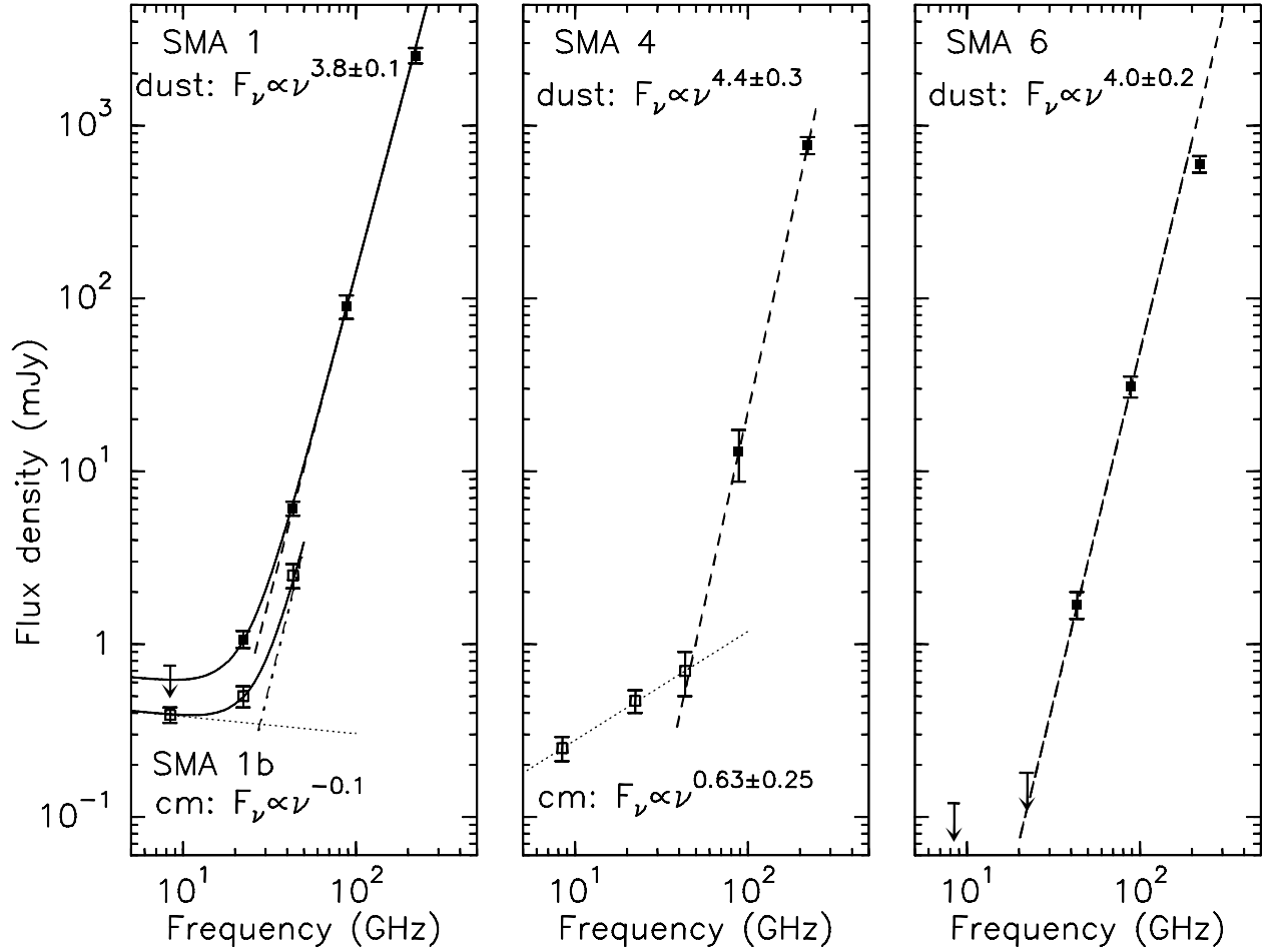
Fig. 13.— Spectral energy distributions for sources SMA1, SMA4, and SMA6. For SMA1, the sum of the emission of SMA1a,b,c, and d are shown as solid squares, while the flux density as a function of frequency for SMA1b is shown as open squares for \nu \leq 43 GHz. Open squares are also used for the \nu \leq 43 GHz emission for SMA4 to indicate that they may not be from the same source as the higher frequency data, the fits in this case assume case 3 described in S4.5.1. Emission models from dust are shown as dashed (or dot-dash in the case of SMA1b) lines, while emission models for free-free emission are shown as dotted lines. For SMA1 the sum of the dust and free-free emission models, described in detail in §4.4.1, is shown as a solid line.
