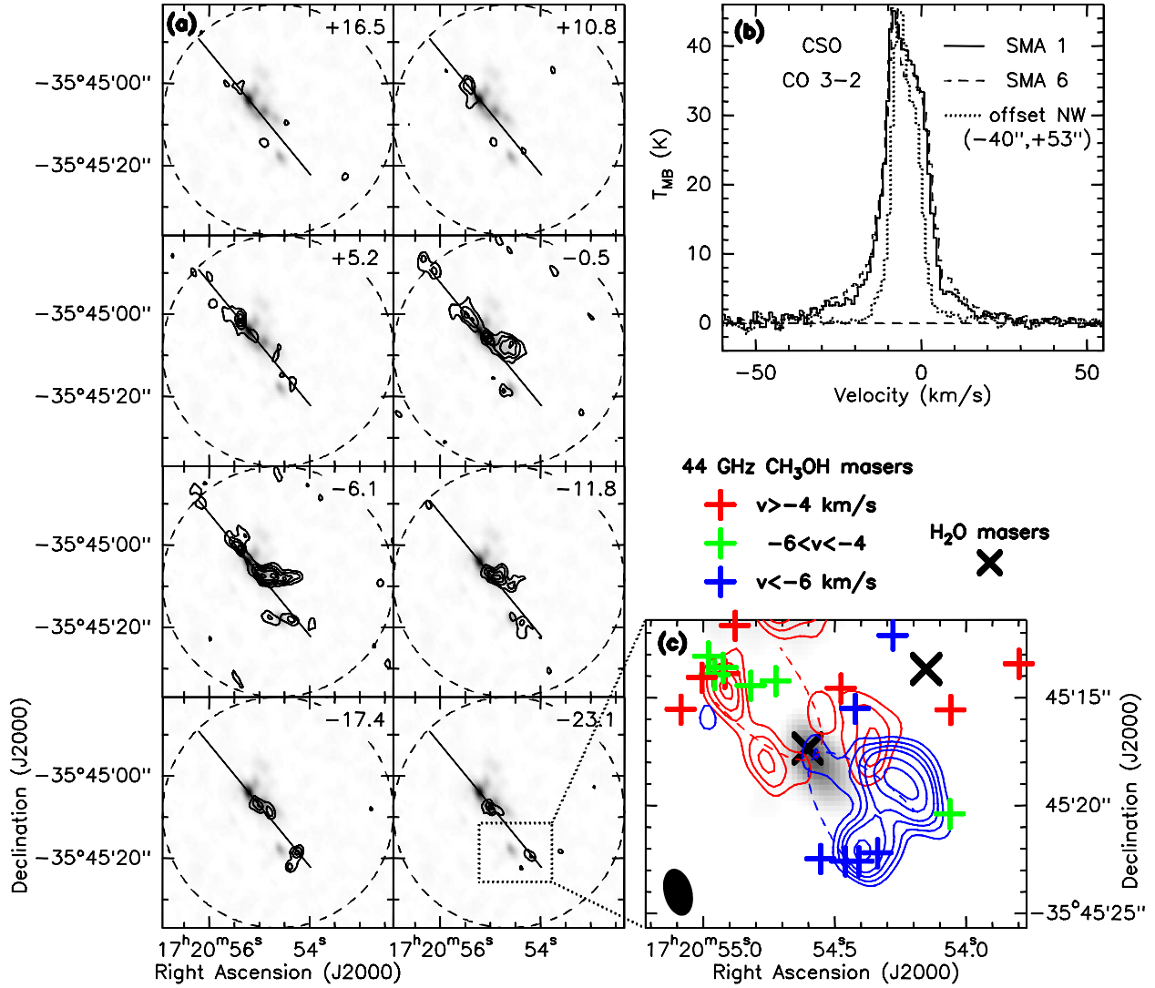
Fig. 7.— (a) Channel maps of SiO 5–4. In each panel, the greyscale is the 1.3 mm continuum emission and the contours are SiO emission (levels = 0.29, 0.48, 0.67, 0.86, 1.05 Jy). The outflow axis is drawn at position angle +39^\circ . The dashed circle is the SMA primary beam. (b) CSO CO (3–2) spectra taken near SMA1, SMA6 and a position offset -40'' , +53'' to the northwest (away from any obvious outflow emission). The SMA1 spectrum was taken 2.9'' from SMA1, and the SMA6 spectrum is the average of the three spectra taken closest to SMA6 ( 5'' , 7'' , and 8'' away). (c) Close up of SiO (5–4) outflow around SMA6. The contours show SiO (5–4) integrated emission, red contours show integrated intensity from +17 to -6 km s ^{-1} and blue contours show integrated intensity from from -8 to -31 km s ^{-1} . The CH 3 OH and H 2 O maser positions are also shown. The solid black ellipse is the SMA synthesized beam.
