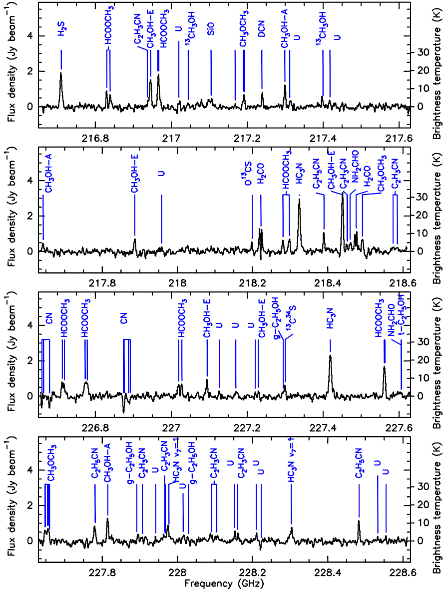
Fig. 5.— SMA spectra of the upper and lower sidebands from the 1.3 mm continuum peak of NGC6334I(N)-SMA1. The spectra have been Hanning smoothed.
