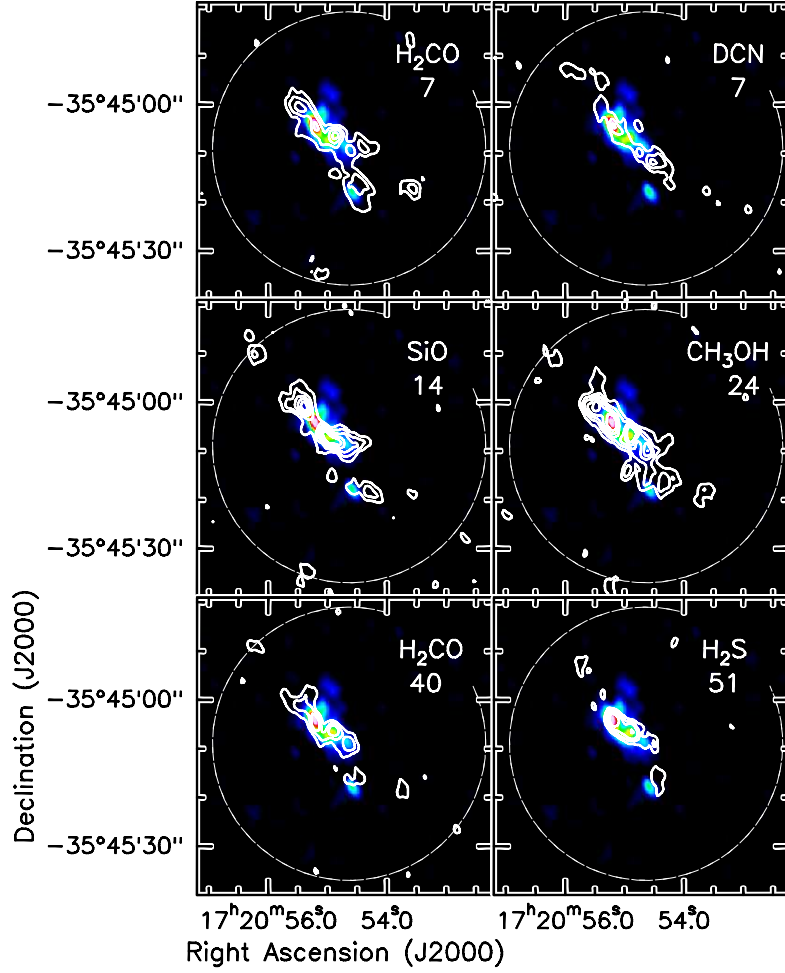
Fig. 6.— In each panel, the colorscale is the 1.3 mm continuum and the contours show the integrated intensity of the indicated spectral lines. The dashed circle is the FWHM of the SMA primary beam; these images have not been corrected for primary beam attenuation. The contour levels are \text{H}_2\text{CO} ( 3_{0,3} - 2_{0,2} ): 4.35, 7.25, 10.15, 13.05 \text{Jy km s}^{-1} ; DCN: 1.77, 2.95, 4.13 \text{Jy km s}^{-1} ; SiO: 6, 10, 14, 18, 22 \text{Jy km s}^{-1} ; \text{CH}_3\text{OH-E} ( 4_{+2,2} - 3_{+1,2} ): 4.8, 8, 11.2, 14.4, 17.6 \text{Jy km s}^{-1} ; \text{H}_2\text{CO} ( 3_{2,2} - 2_{2,1} ): 3.24, 5.4, 7.56 \text{Jy km s}^{-1} ; \text{H}_2\text{S} : 2.55, 4.25, 5.95, 9.35 \text{Jy km s}^{-1} . The number below each molecular name is the E_{\text{lower}} of the transition in units of \text{cm}^{-1} .
