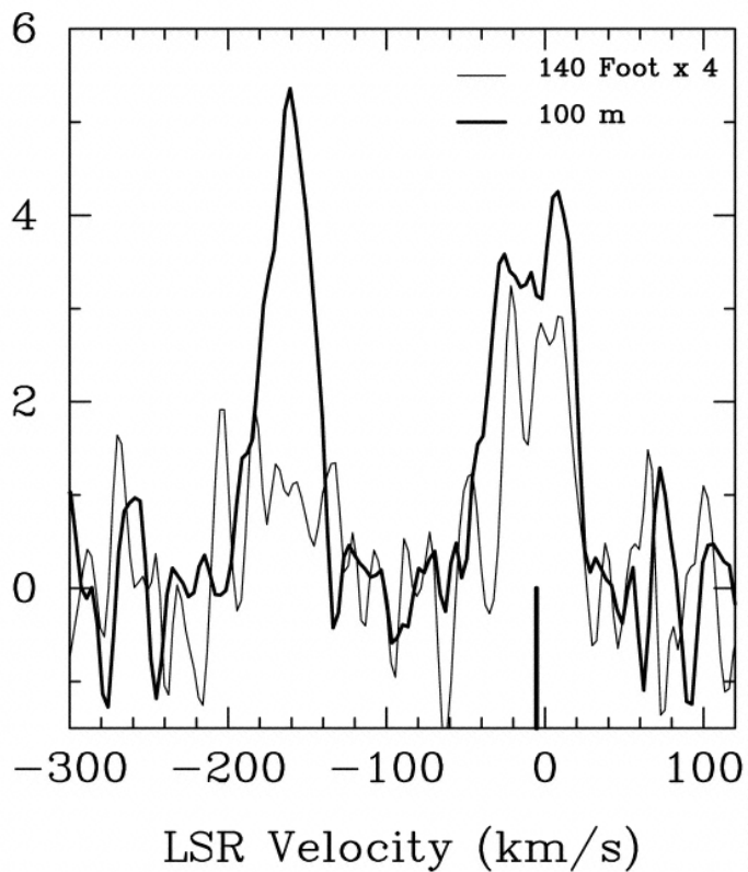
^3\text{He}^+ line at 8665 MHz
