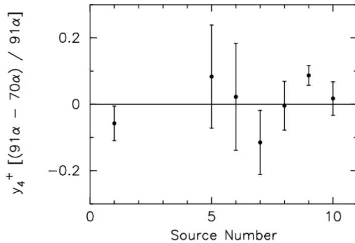
10 HII Regions
