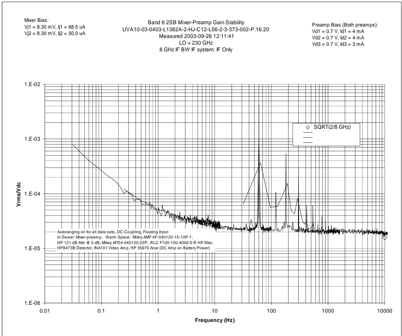
Figure 3: Spectral Density for IF System
