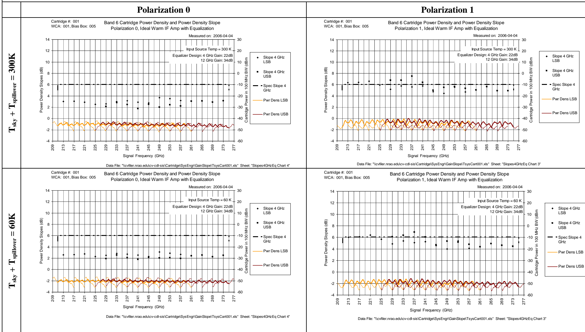
Figure 6: Gain Slope in 4 GHz IF Bandwidth, Assuming Equalizers in Warm IF Amps
