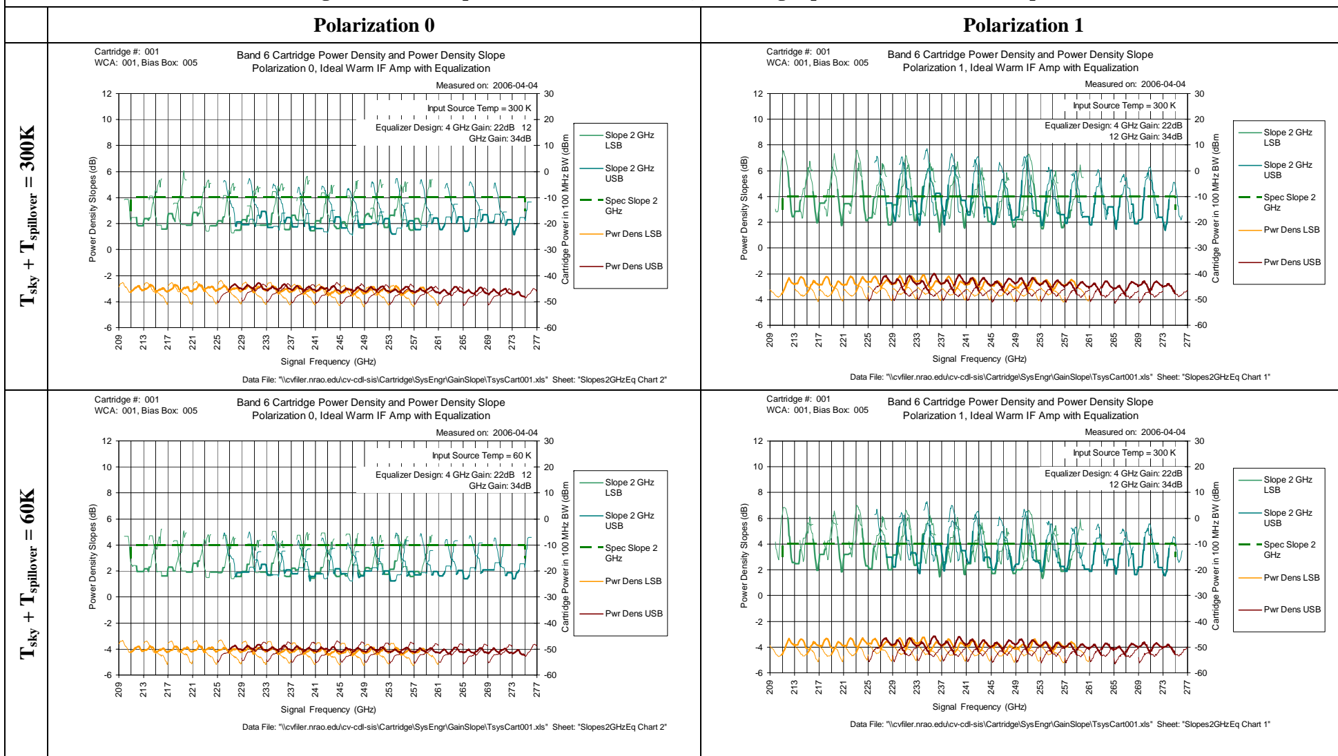
Figure 5: Gain Slope in 2 GHz IF Bandwidth, Assuming Equalizers in Warm IF Amps
