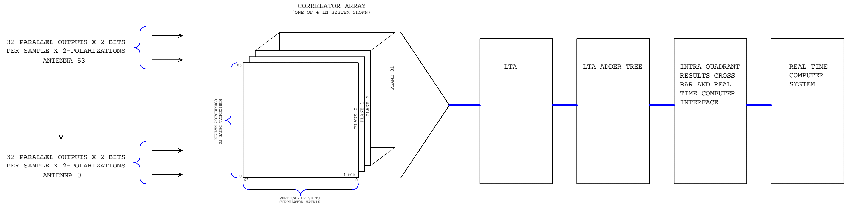
ALMA CORRELATOR BLOCK DIAGRAM
