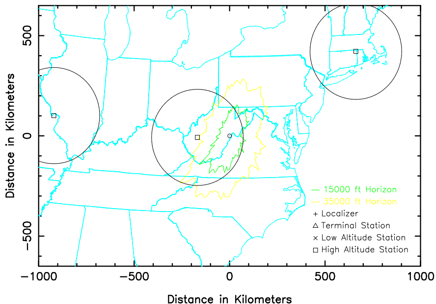
Figure 9: The locations of DME channel 121 (1144 MHz) stations. The high altitude stations show 240 km range circles. The low altitude station show 74 km radius circles, the terminal stations are enclosed in 46 km radius circles, and the localizer stations are drawn with 20 km radius circles. The irregular contours around Green Bank show the line-of-sight horizons of the GBT prime focus point for two different aircraft altitudes.
