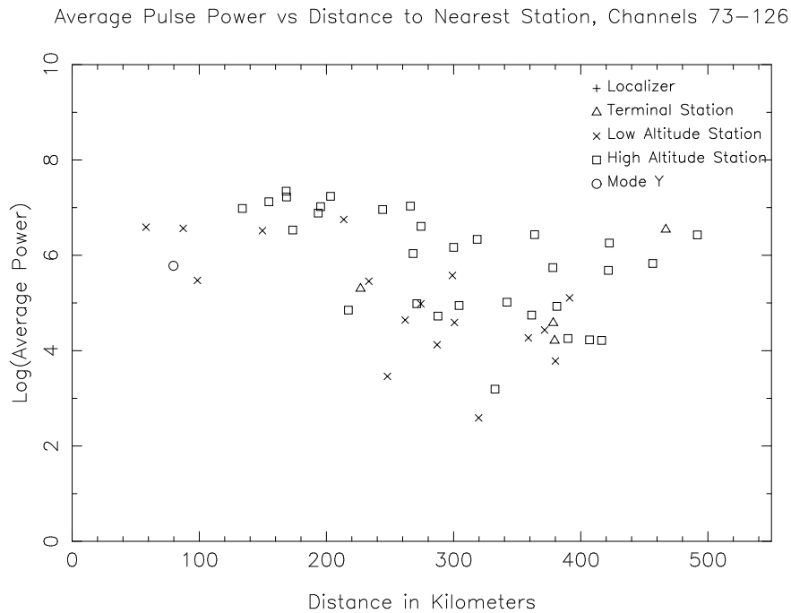
Figure 13: Relative average signal power in five minutes as a function of the distance to the nearest DME station from Green Bank for all DME channels above 1100 MHz shown in Figure 2. The high, low, terminal and localizer station symbols are the same as in Figures 8 and 9.
