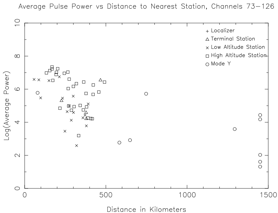
Figure 14: Same as Figure 13 except for a longer distance range. There are very few mode Y stations and few mode Y signals detected so these are given a separate symbol. No stations were listed in the NACO database for five of the mode Y channels in which signals were detected. These are plotted on the right side of the figure.
