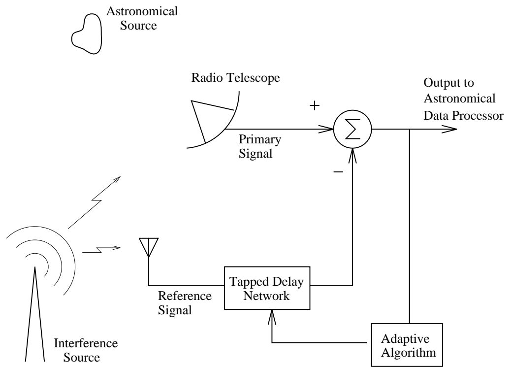
Figure 1. Basic adaptive cancellation scheme.
