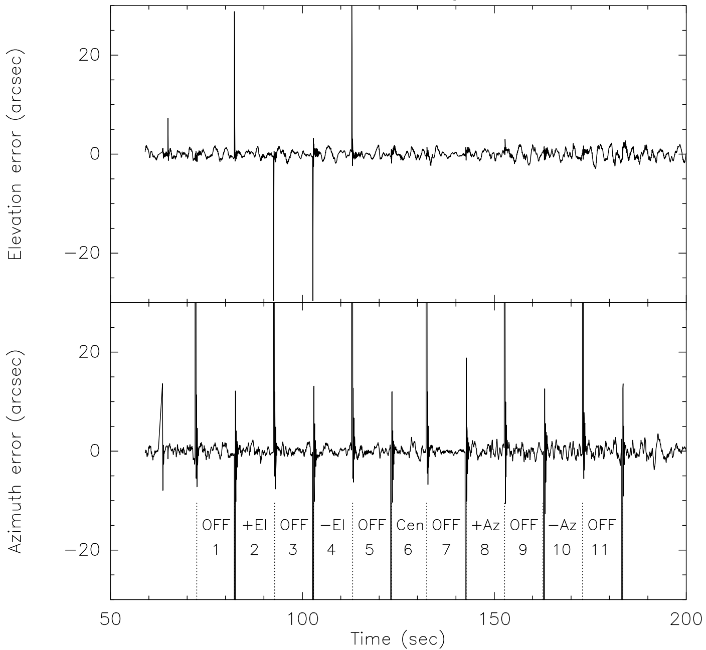
AEC antenna: motions during FivePoint scan
