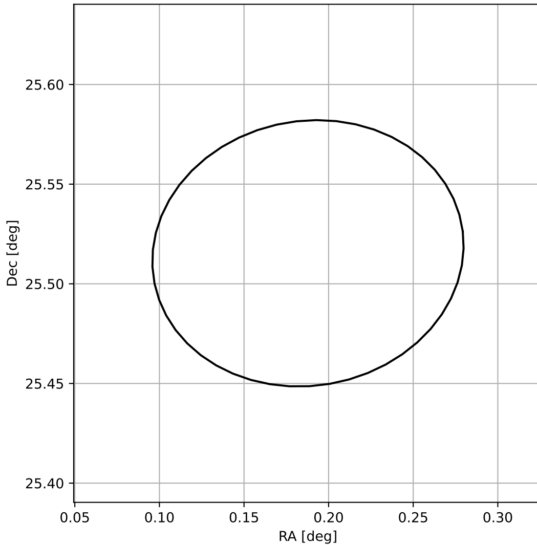
4FGL J0000.7+2530
