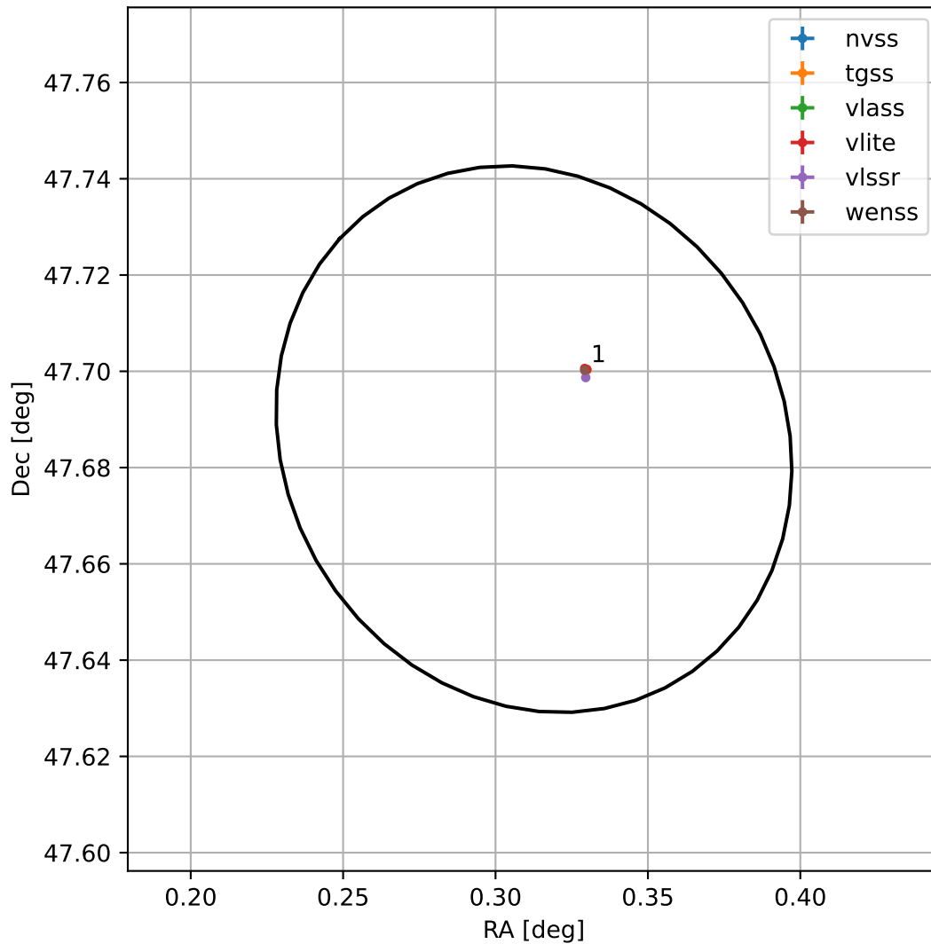
4FGL J0001.2+4741
