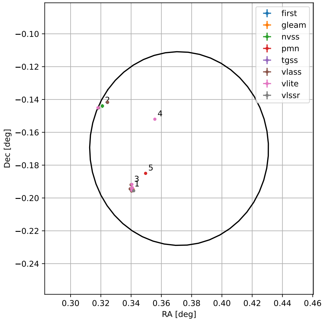
4FGL J0001.4-0010
