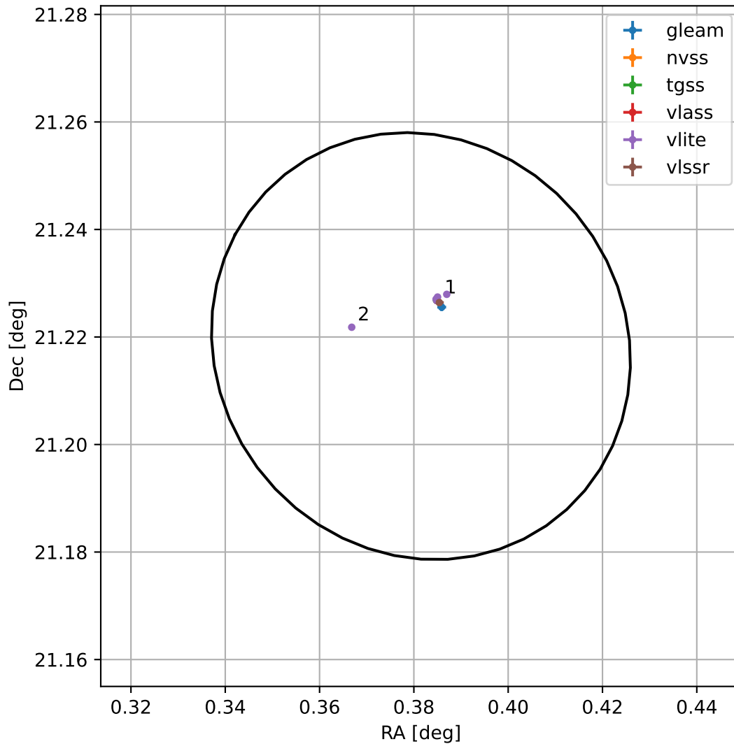
4FGL J0001.5+2113
