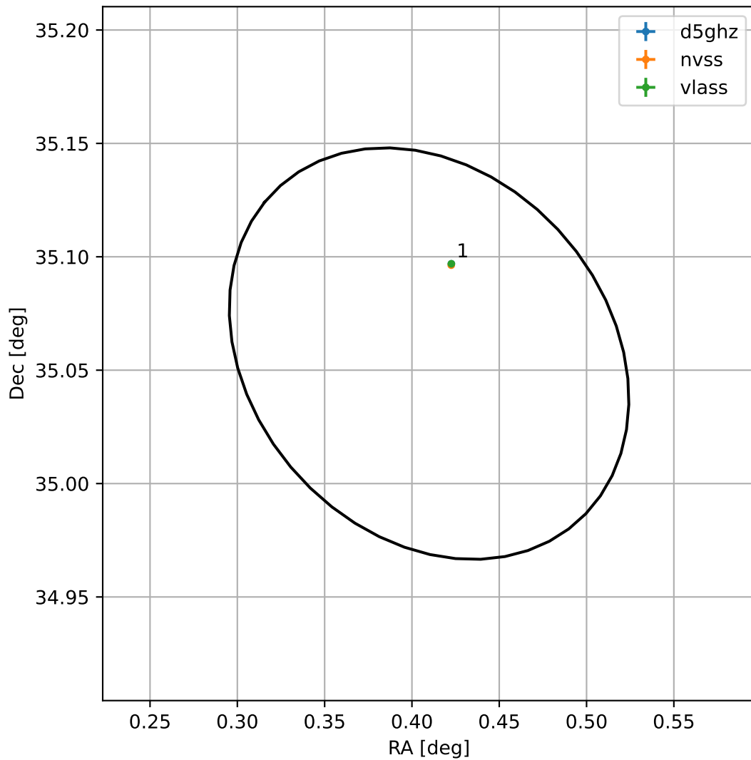
4FGL J0001.6+3503
