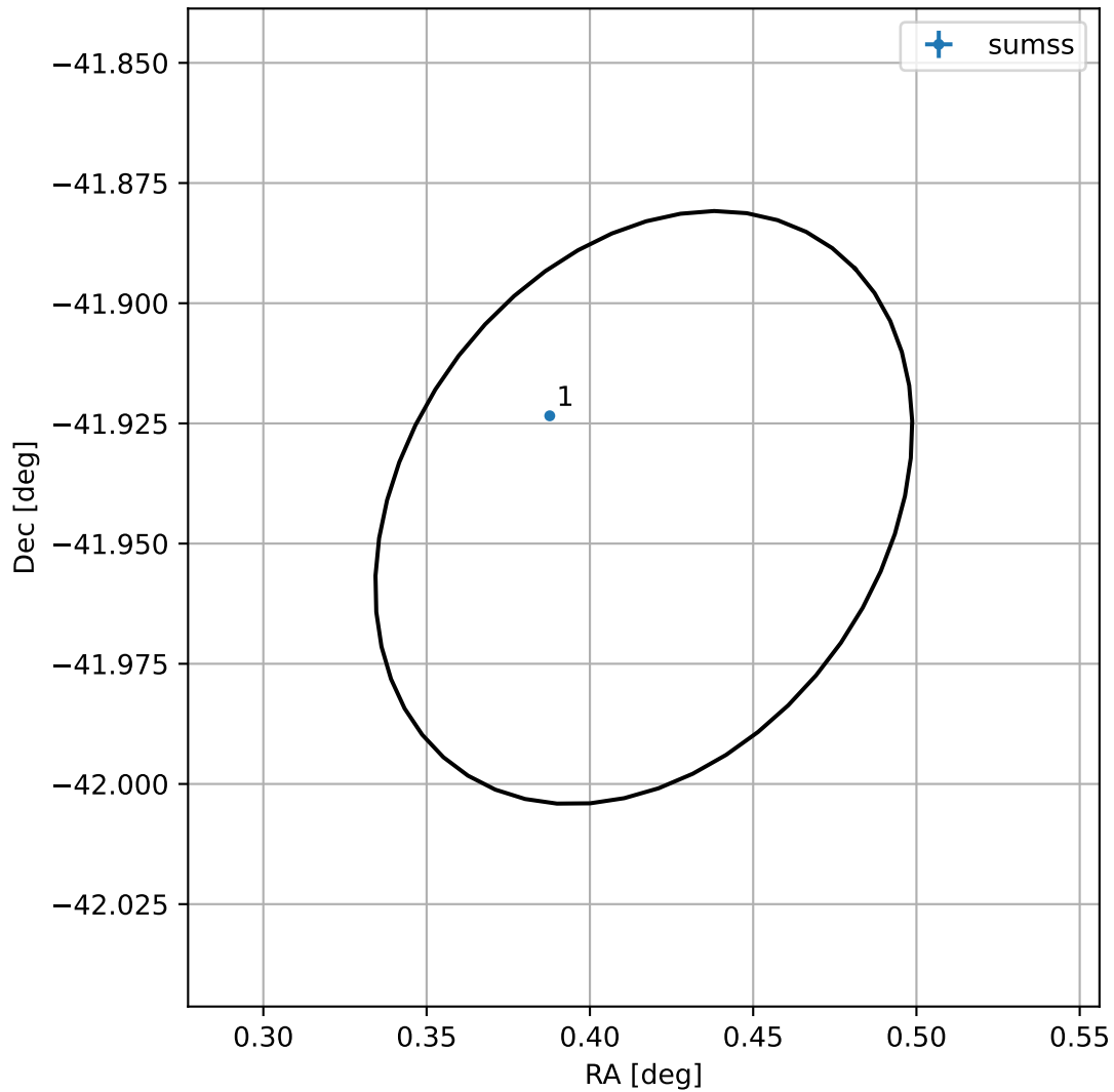
4FGL J0001.6-4156
