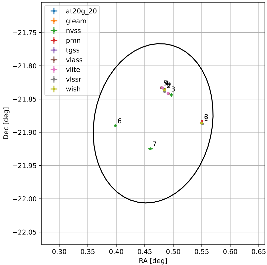
4FGL J0001.8-2153
