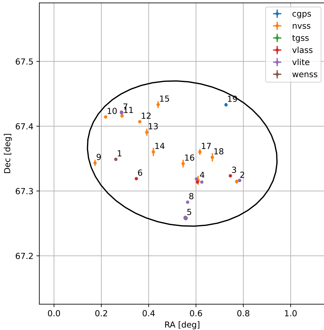
4FGL J0002.1+6721
