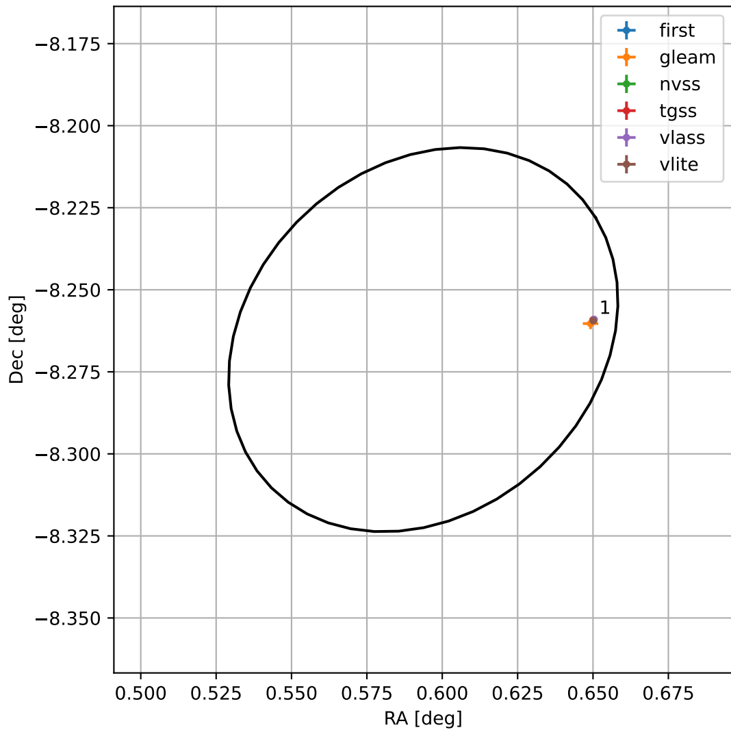
4FGL J0002.3-0815
