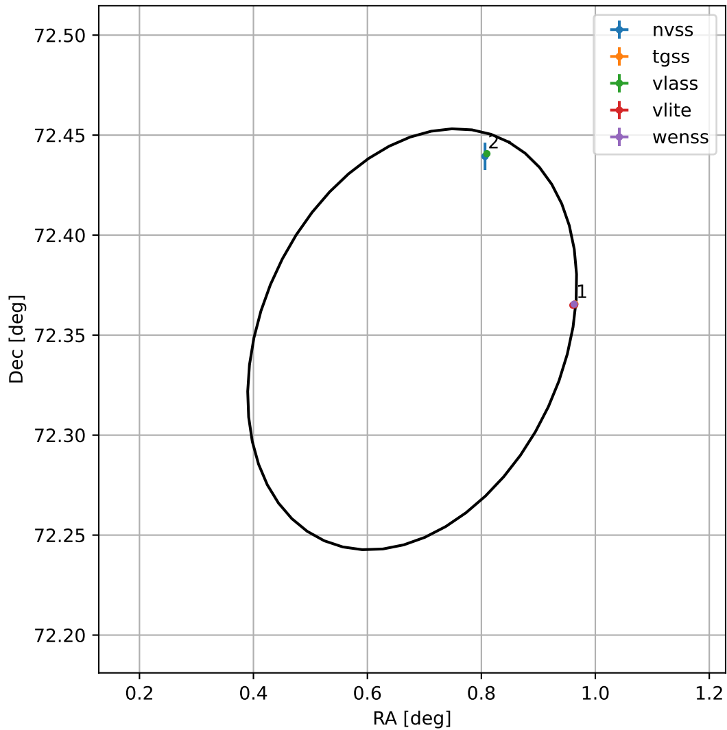
4FGL J0002.7+7220
