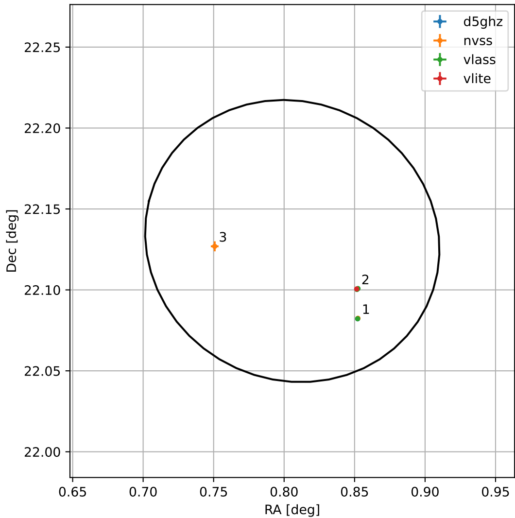
4FGL J0003.2+2207
