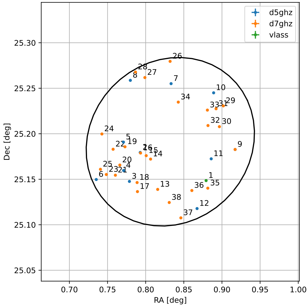
4FGL J0003.3+2511
