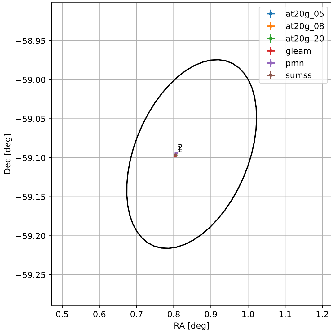
4FGL J0003.3-5905
