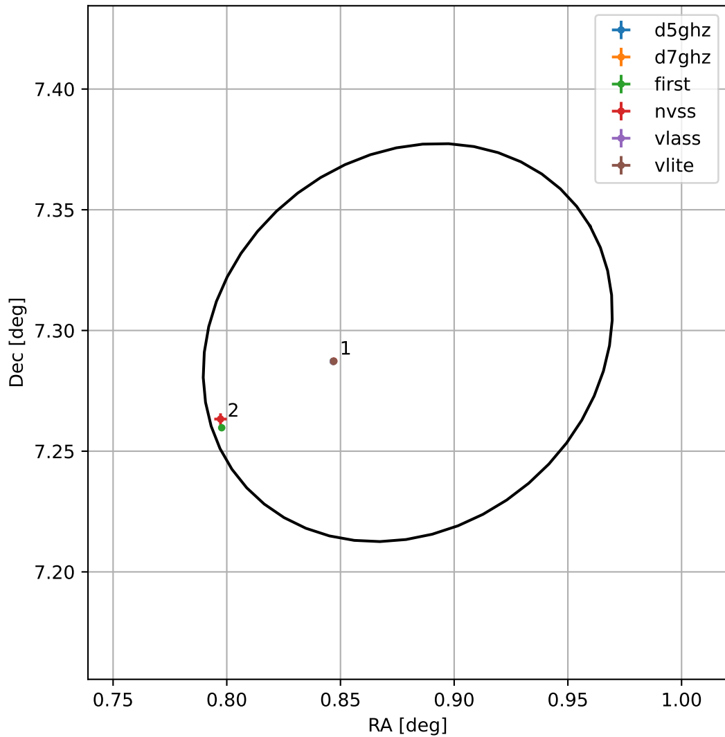
4FGL J0003.5+0717
