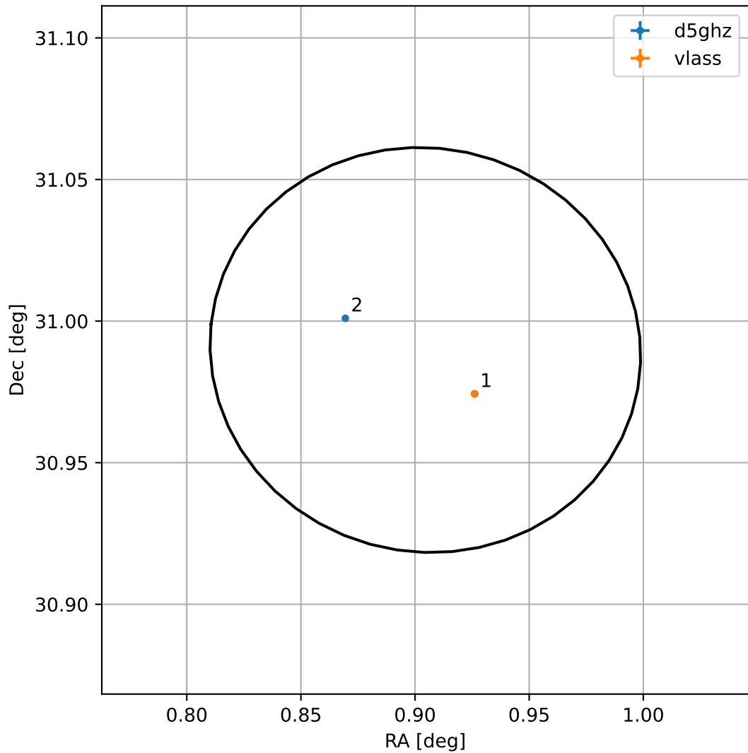
4FGL J0003.6+3059
