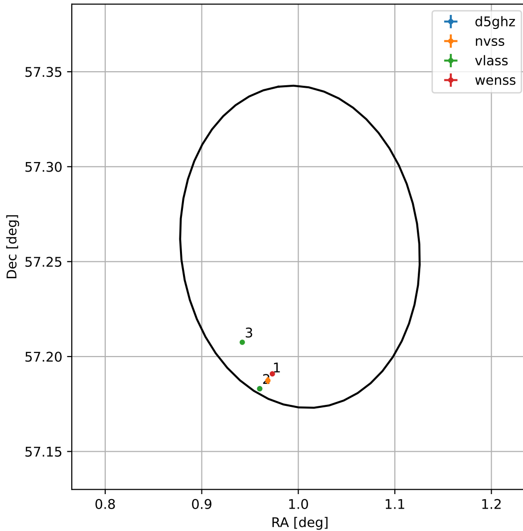
4FGL J0004.0+5715
