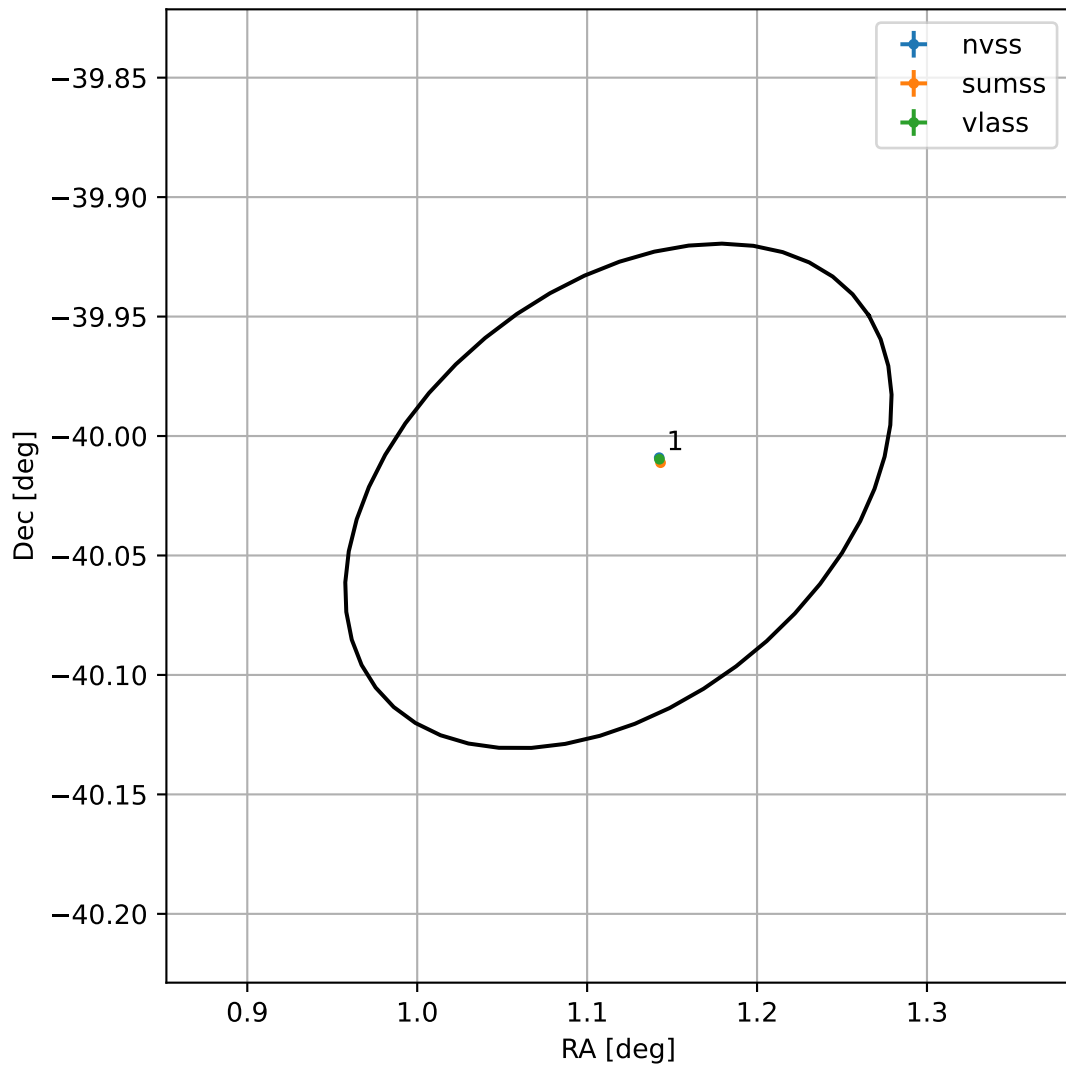
4FGL J0004.4-4001
