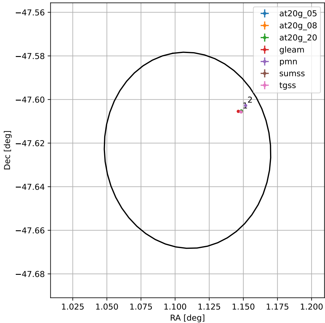
4FGL J0004.4-4737
