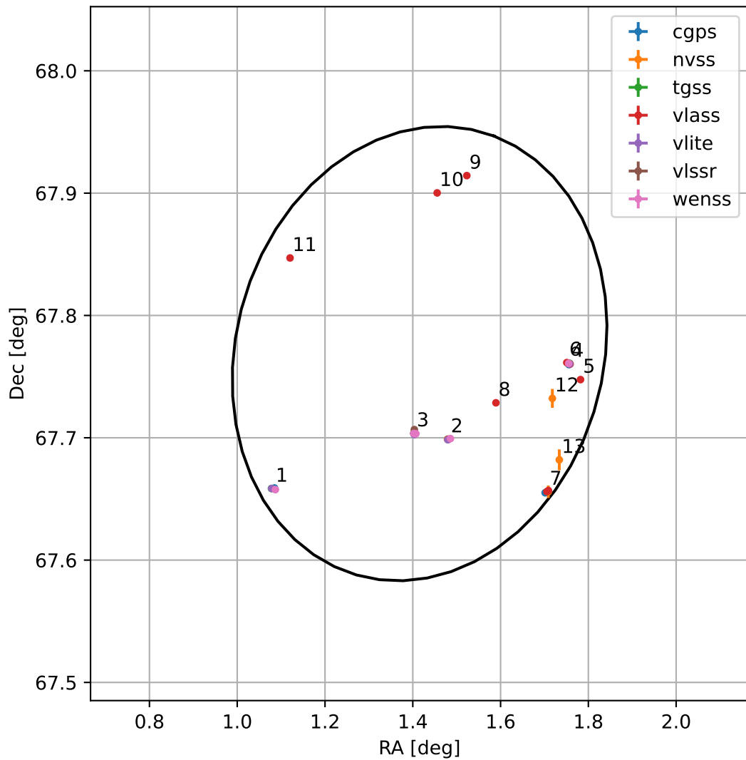
4FGL J0005.6+6746
