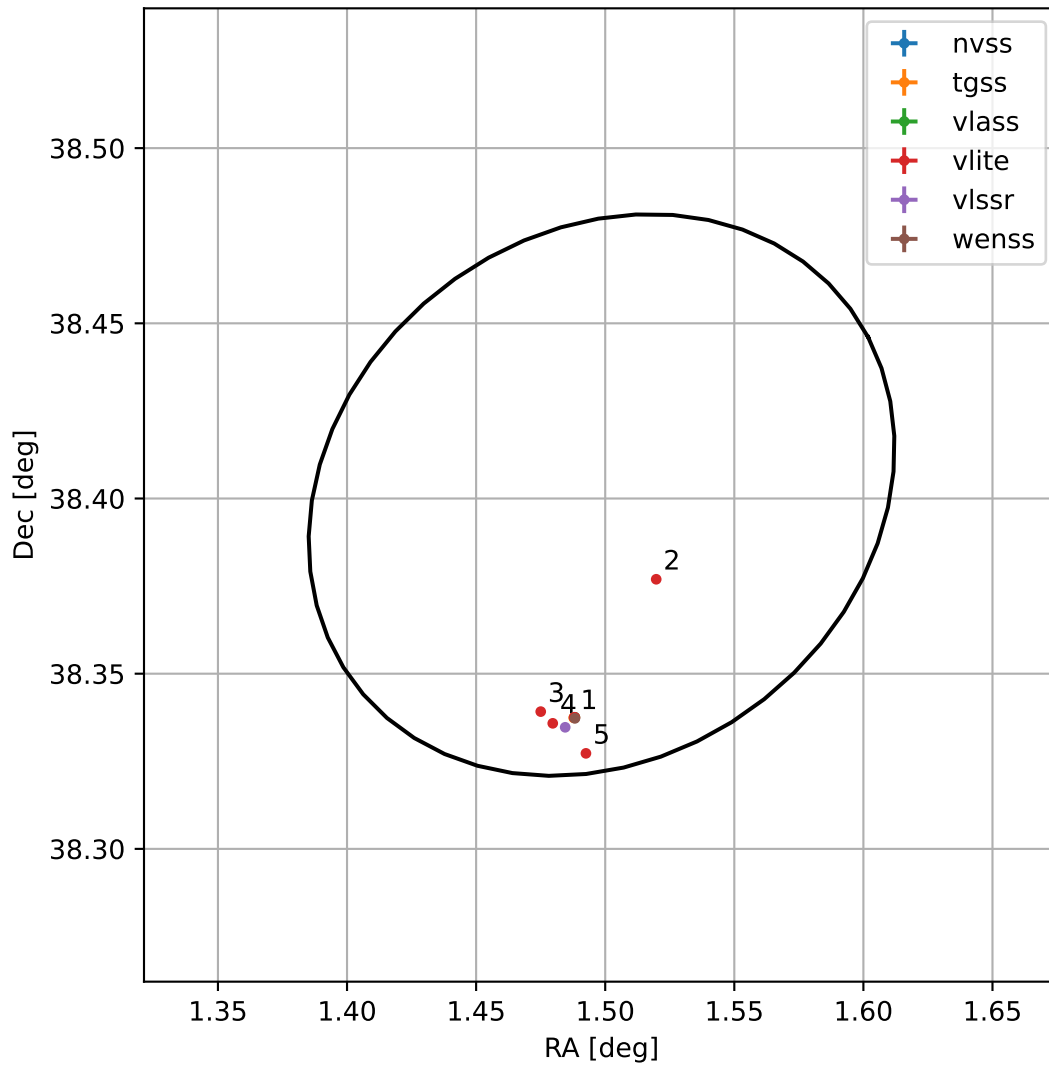
4FGL J0005.9+3824
