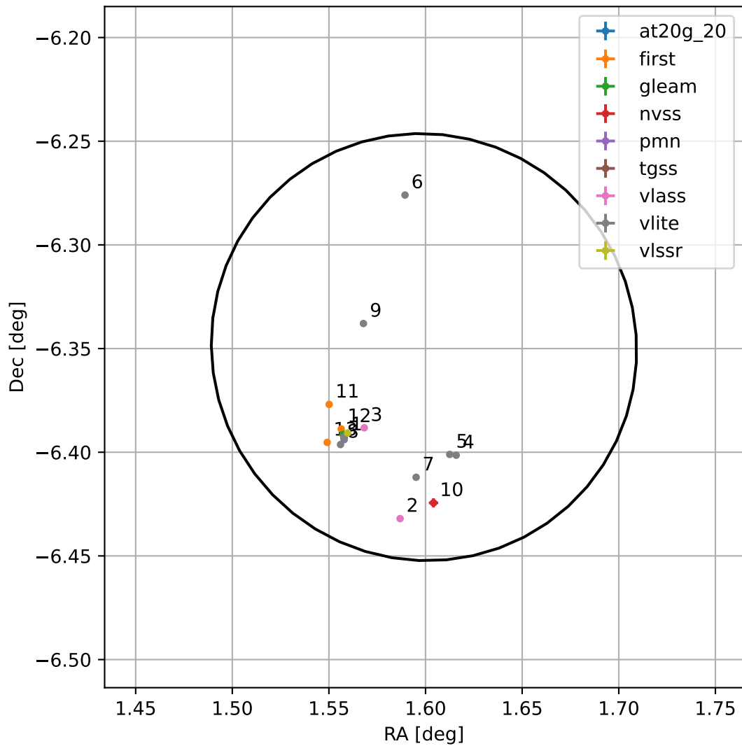
4FGL J0006.3-0620
