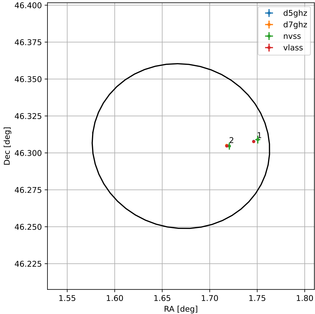
4FGL J0006.6+4618
