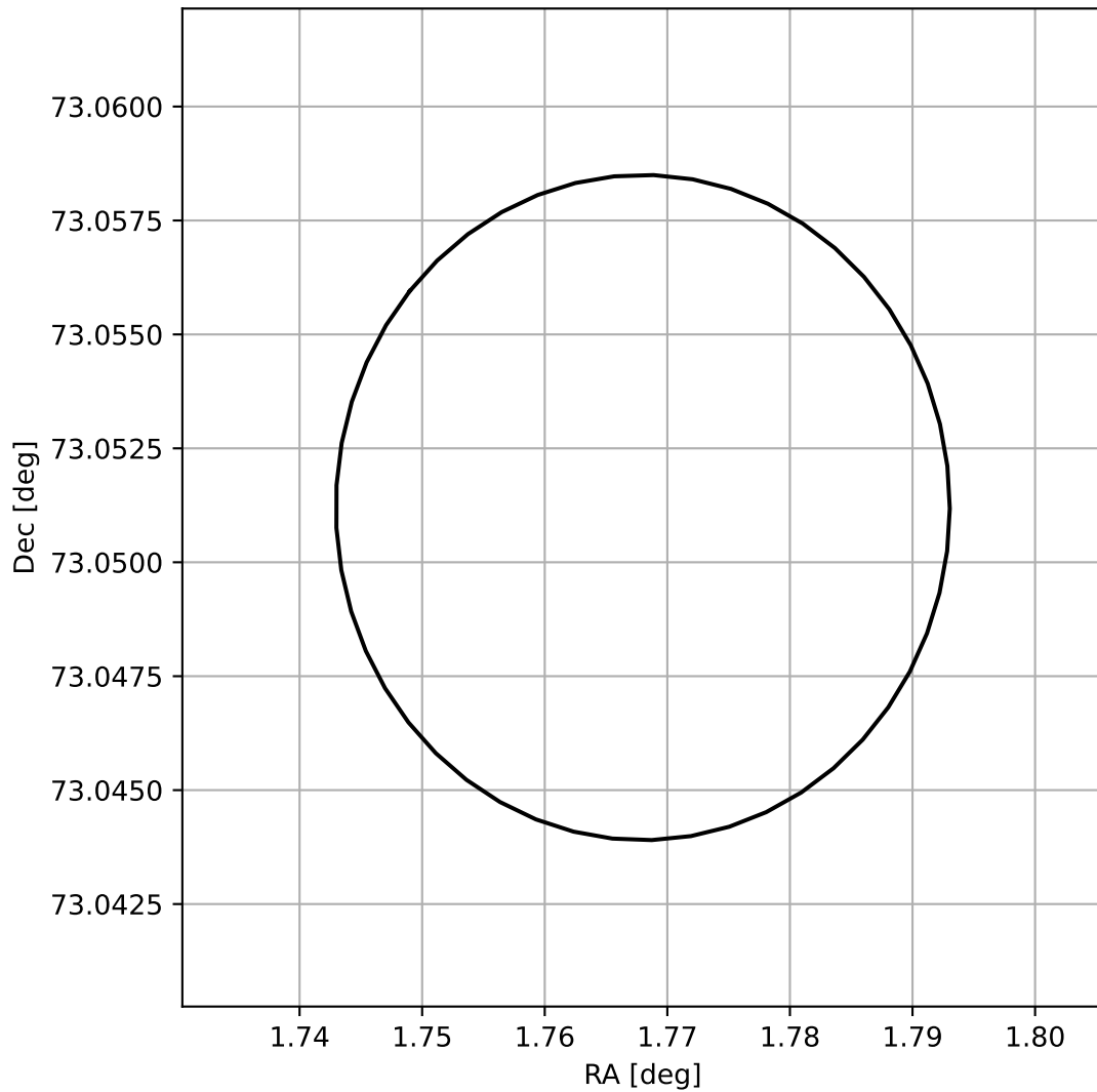
4FGL J0007.0+7303
