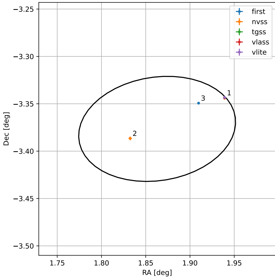
4FGL J0007.4-0322
