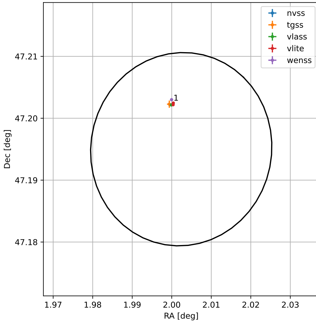
4FGL J0008.0+4711
