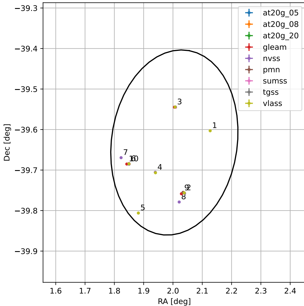
4FGL J0008.0-3937
