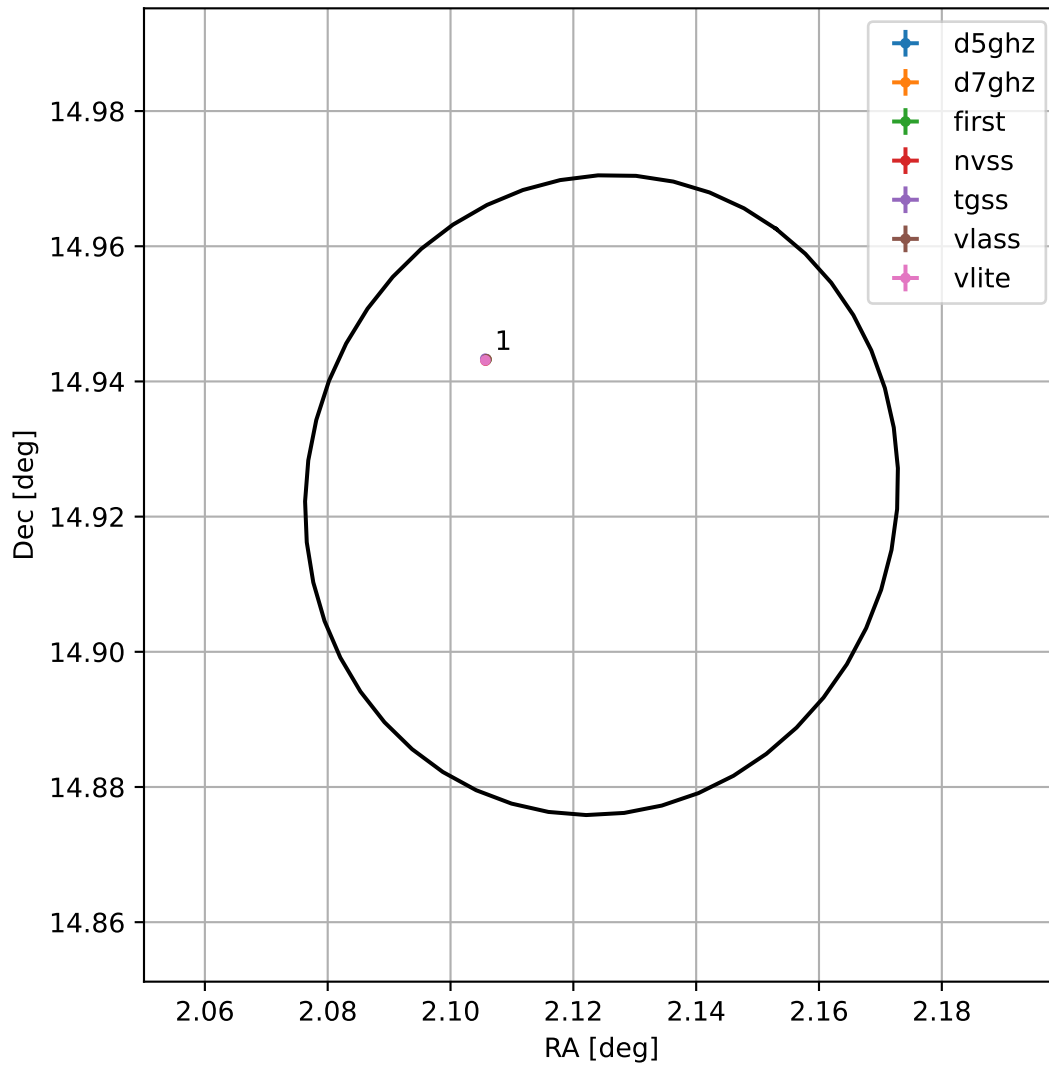
4FGL J0008.4+1455
