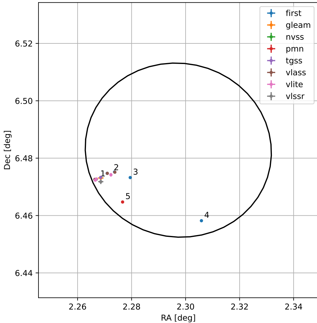
4FGL J0009.1+0628
