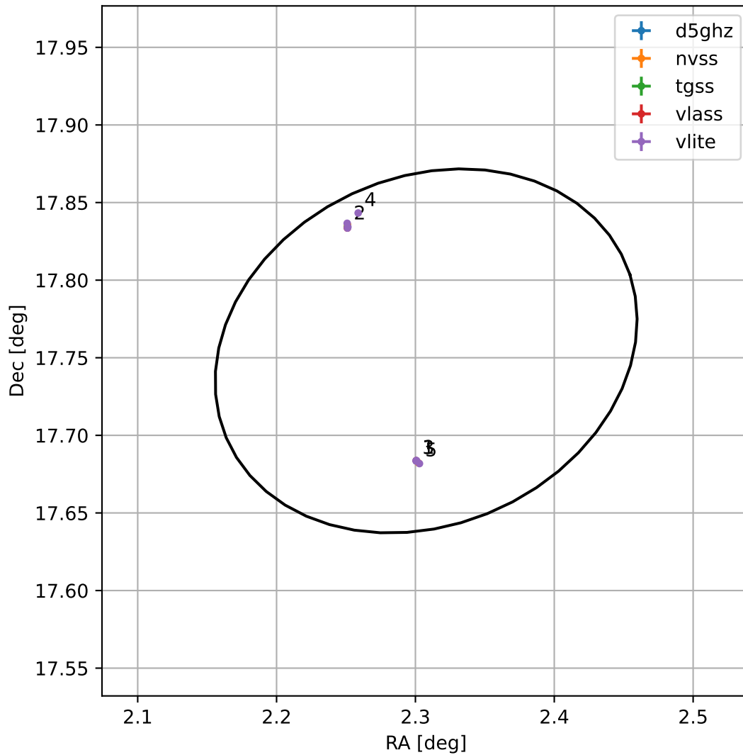
4FGL J0009.2+1745
