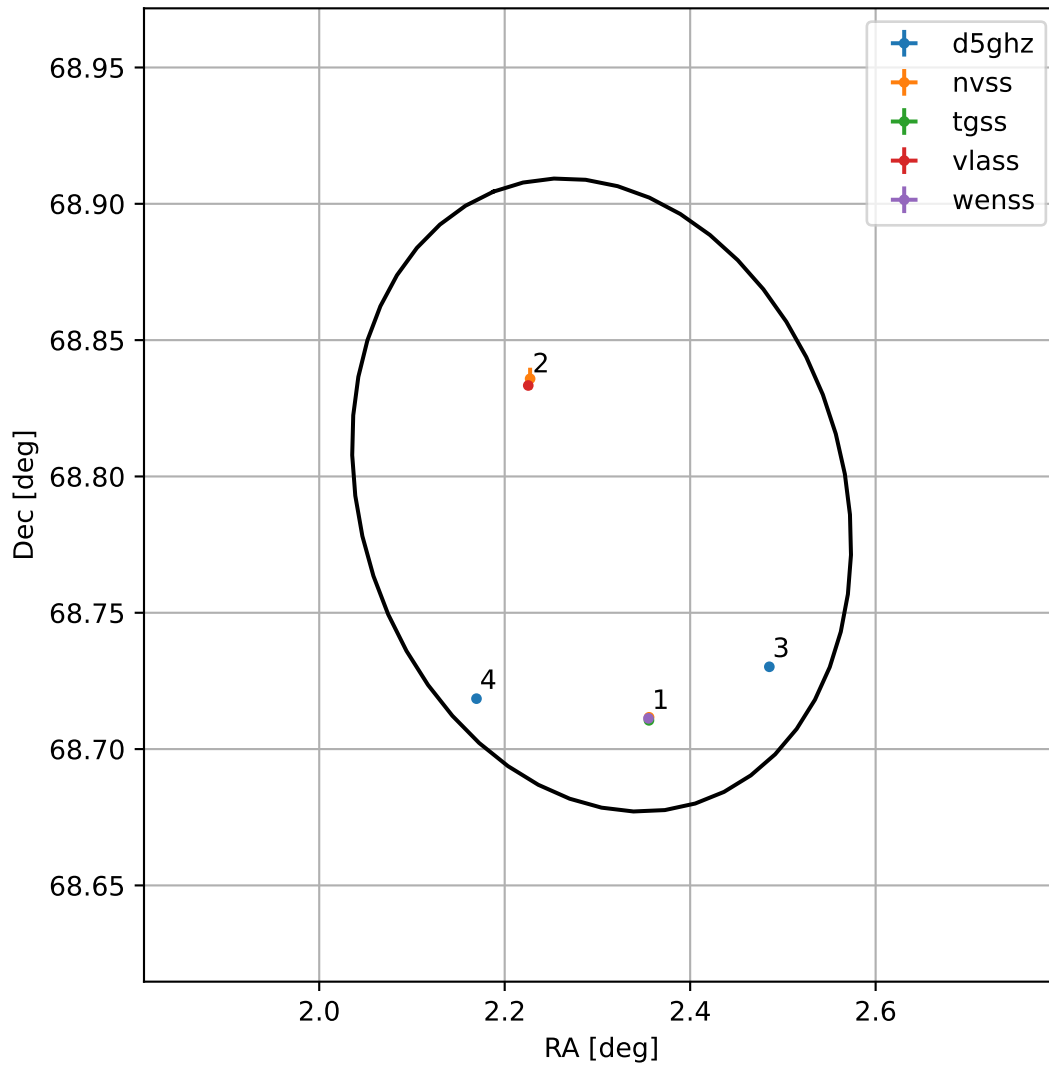
4FGL J0009.2+6847
