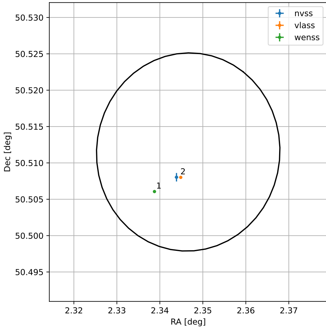
4FGL J0009.3+5030
