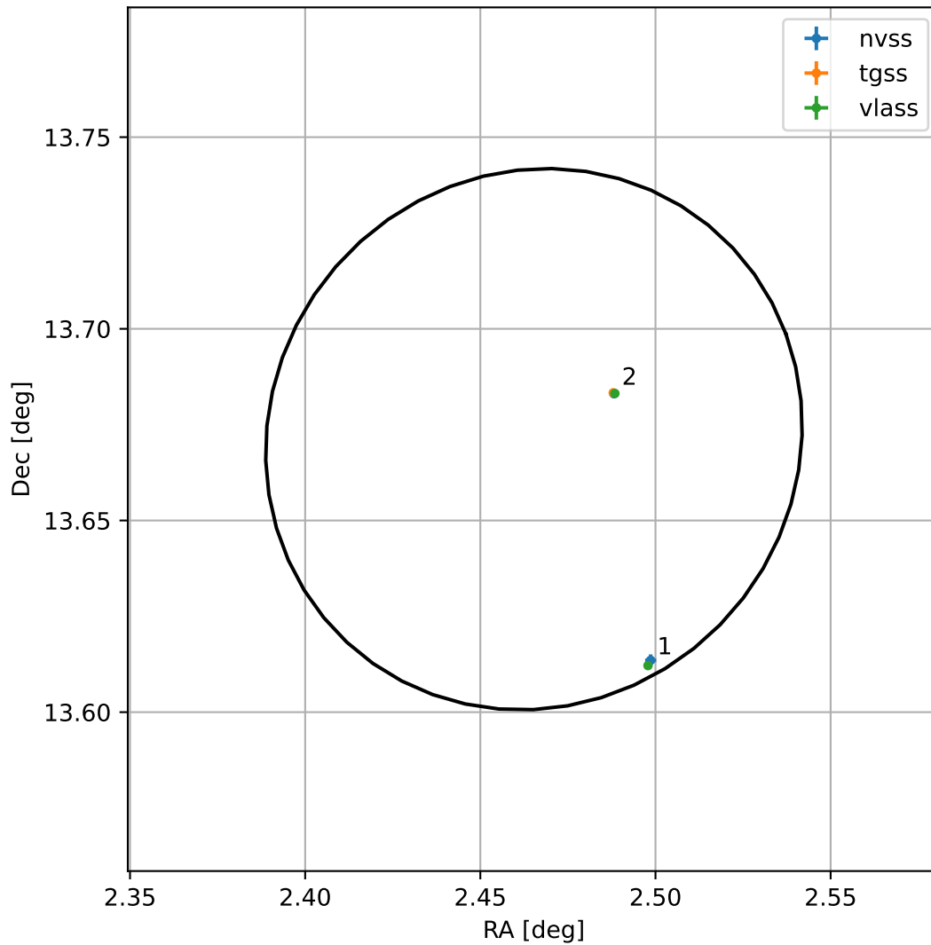
4FGL J0009.8+1340
