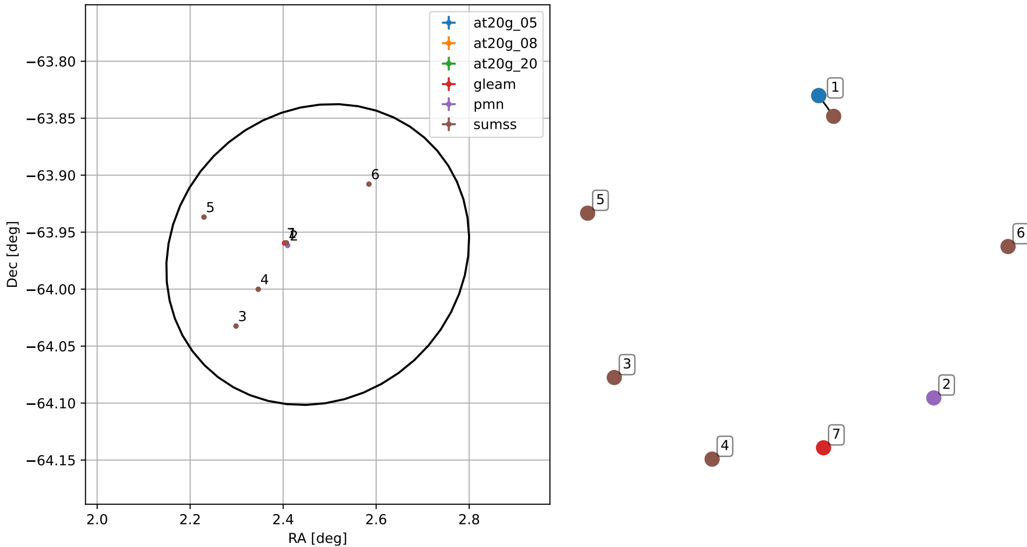
4FGL J0009.8-6358
