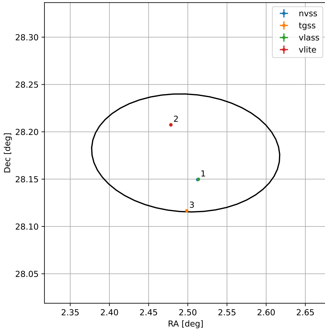
4FGL J0009.9+2810
