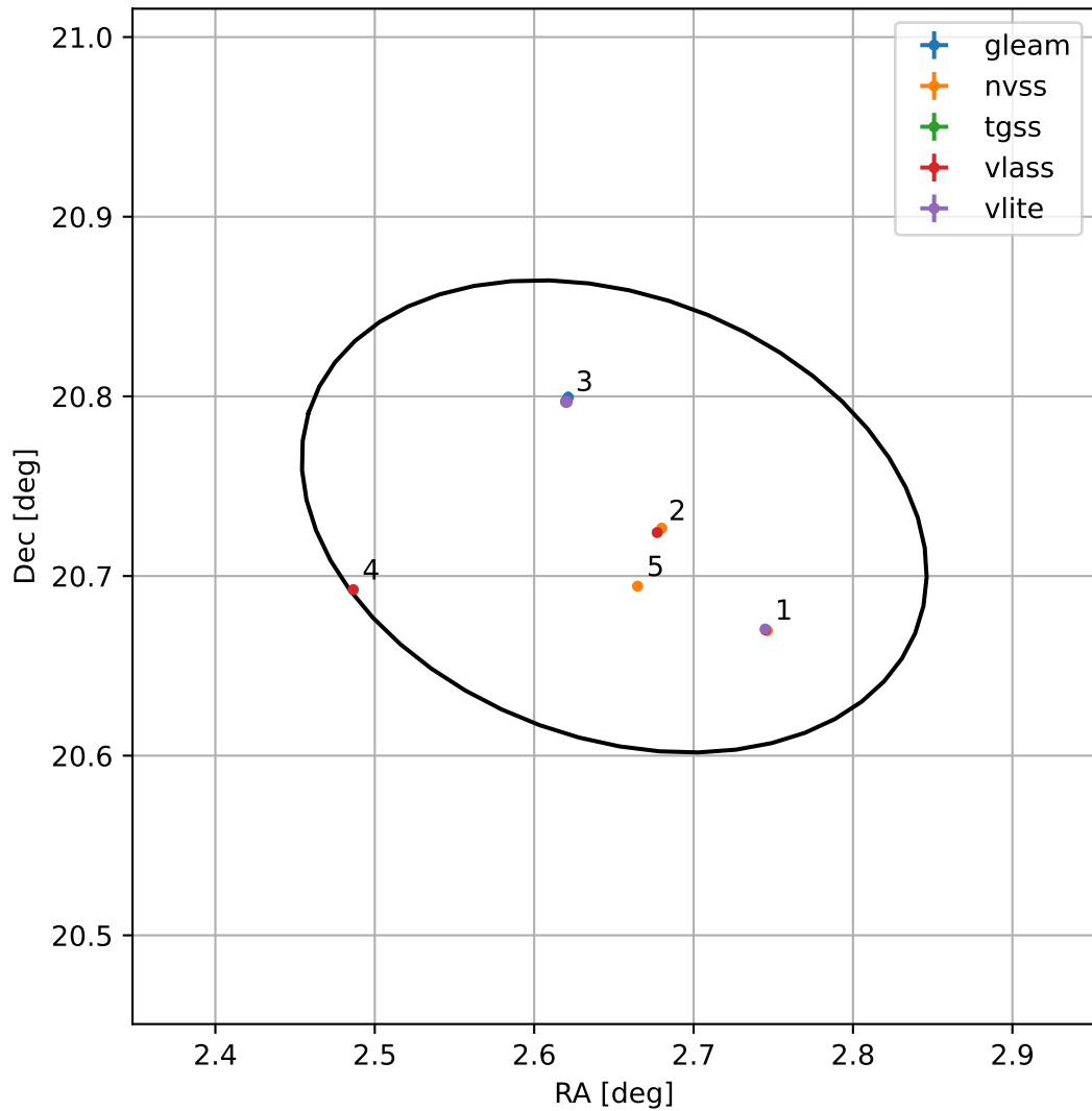
4FGL J0010.6+2043
