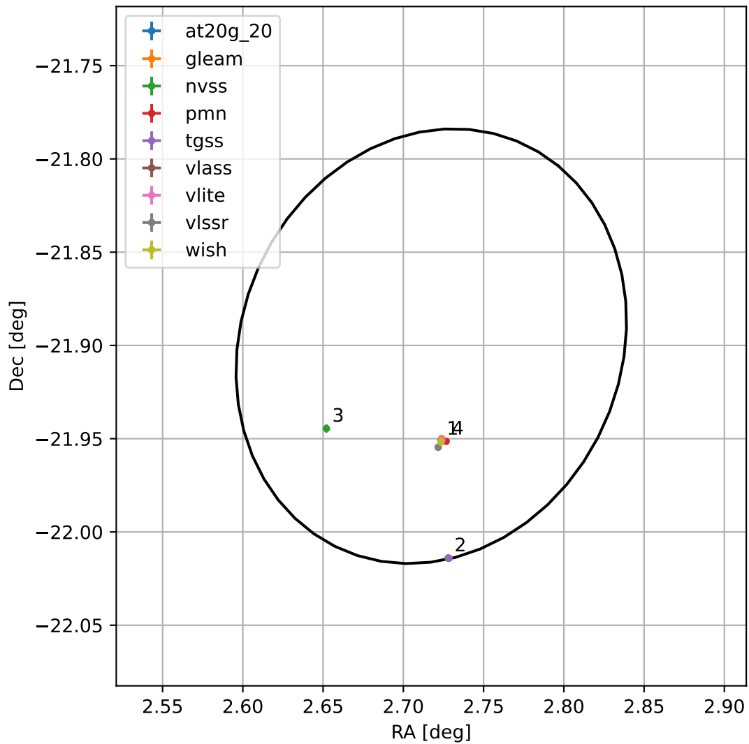
4FGL J0010.8-2154
