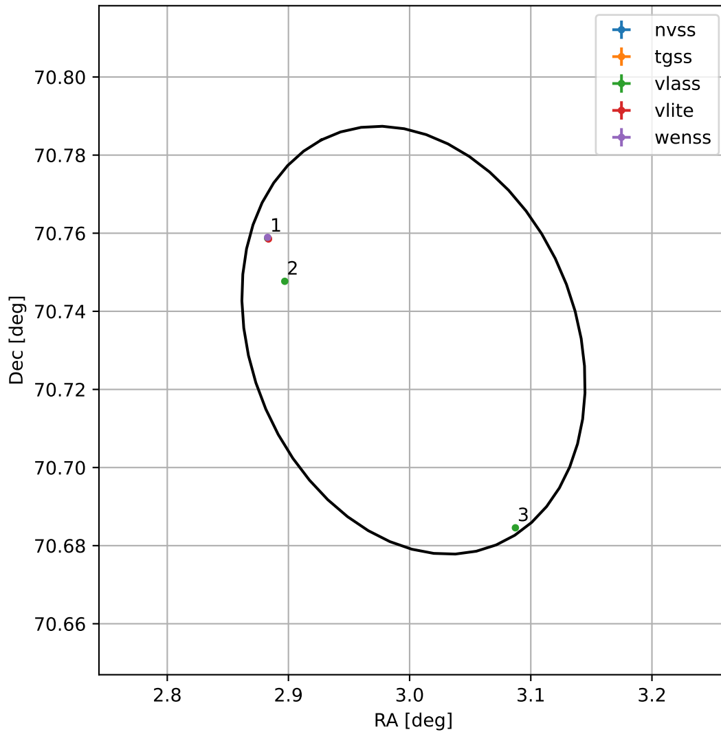
4FGL J0012.0+7043
