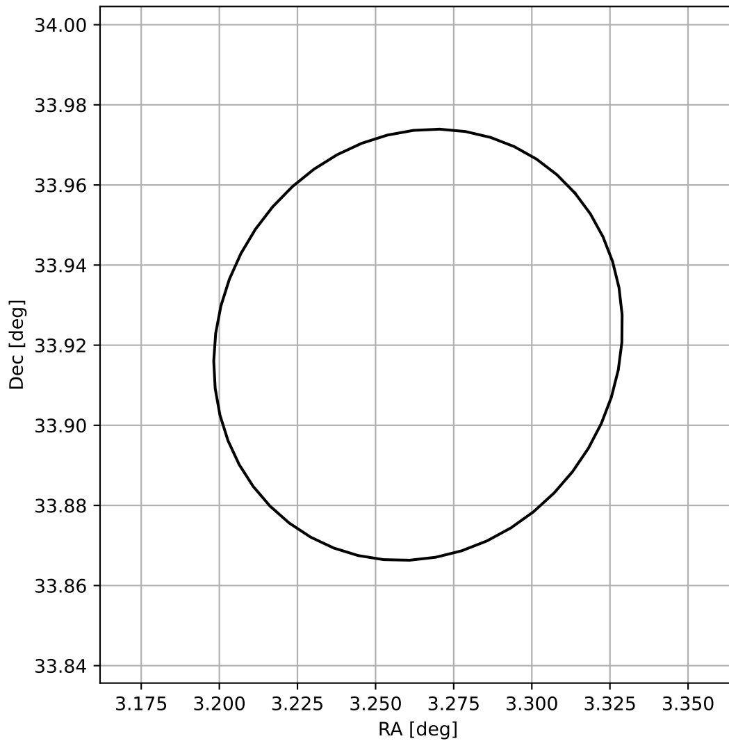
4FGL J0013.0+3355
